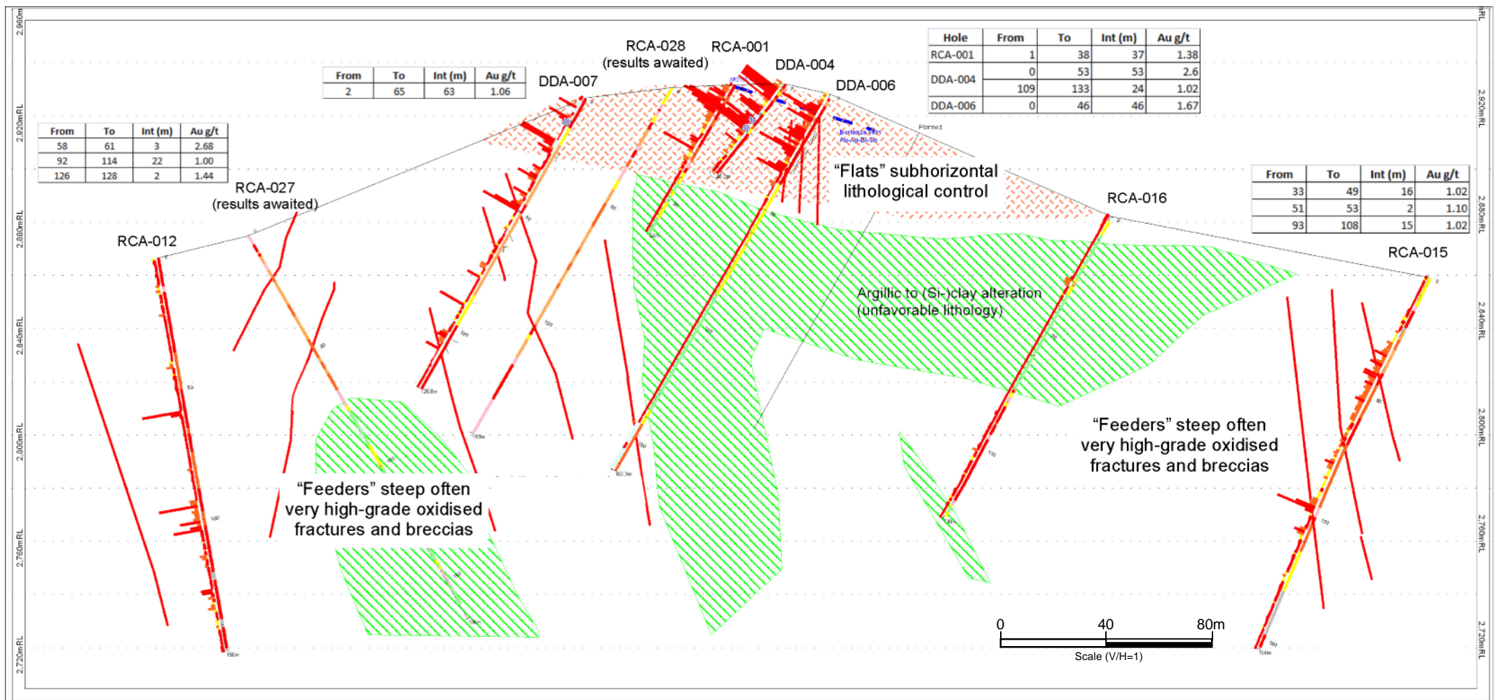
Figure 2. Preliminary interpretative cross-section (see Figure 1 for section location), Amulsar project, Armenia. Broad zones corresponding to “flats” and “feeders” as indicated. Red-shade corresponds to advanced argillic alteration assemblage and green to argillic assemblage.
