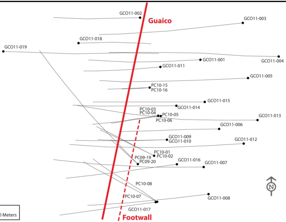
Figure 2 Cisneros Project – Veins at the Guaico Structure
