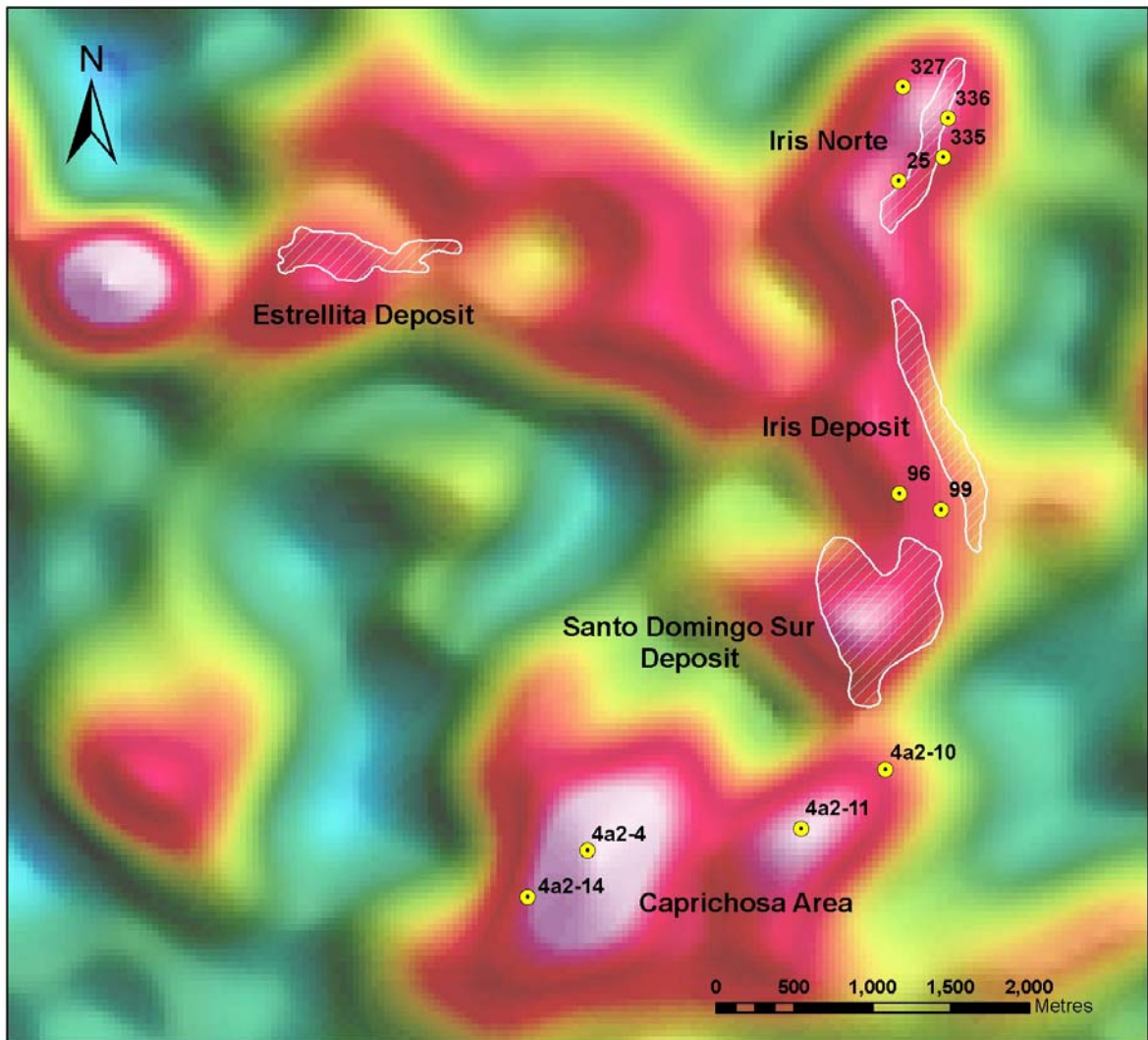
Figure 2: FALCON TEM gravity image showing the location of the copper-iron deposits and mineralized zones on the Santo Domingo Property. The drill holes presented contain significant iron intercepts which are listed in Table 2.
