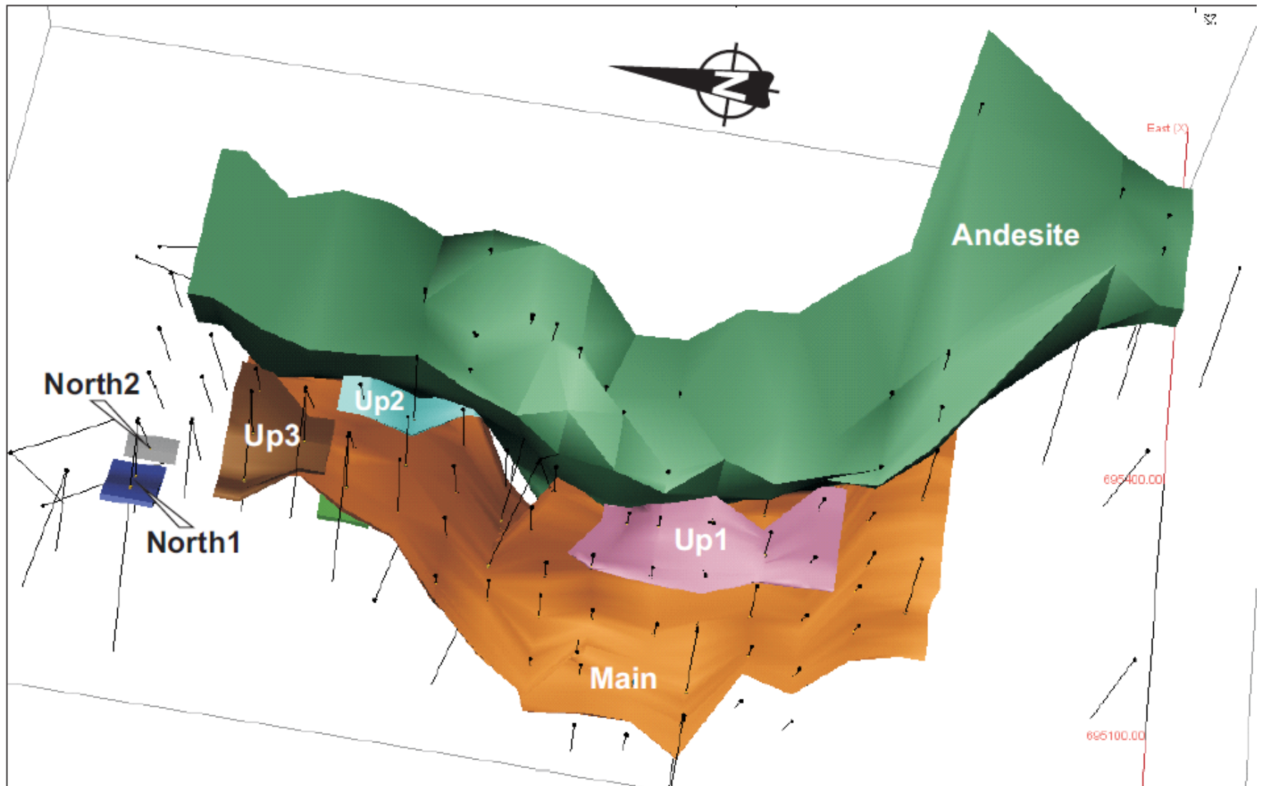
Figure 2: 3D View of El Domo Resource Wireframes
