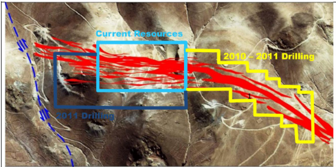
Figure 2: Tajo Vein System, Plan View.
