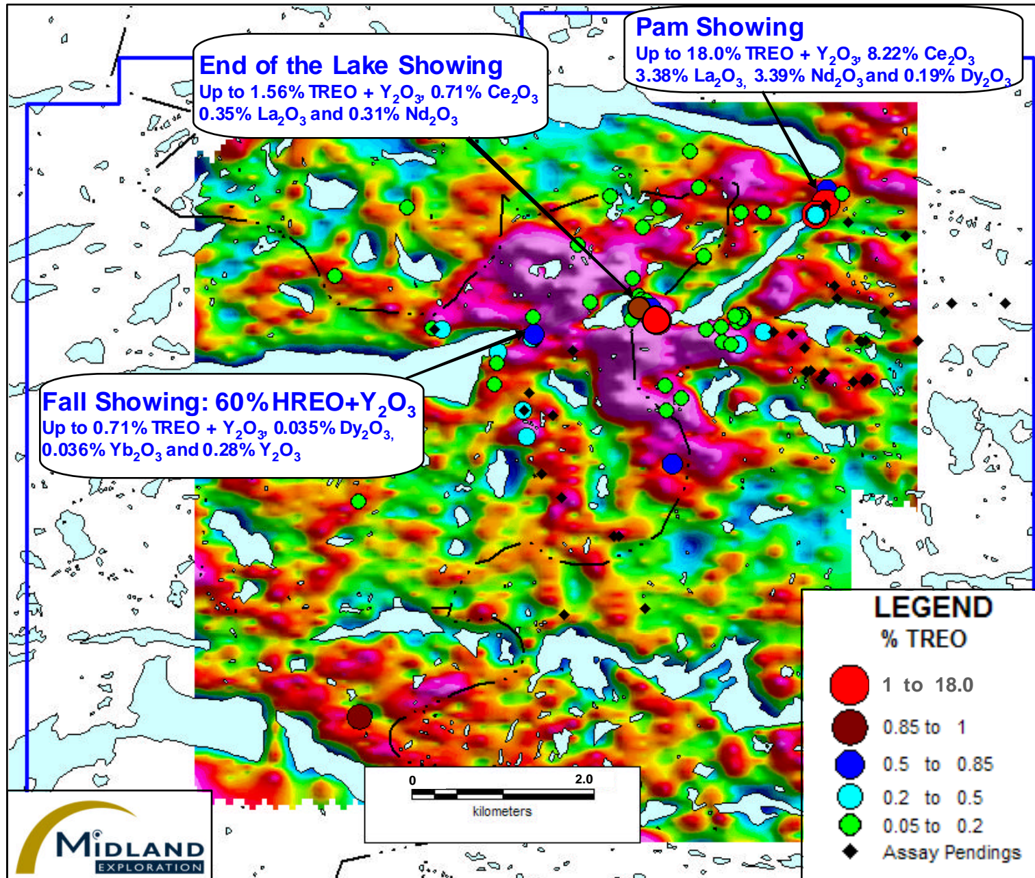
Figure 3. Ytterby 2 Grab Sample Results on Thorium Radiometric Map
