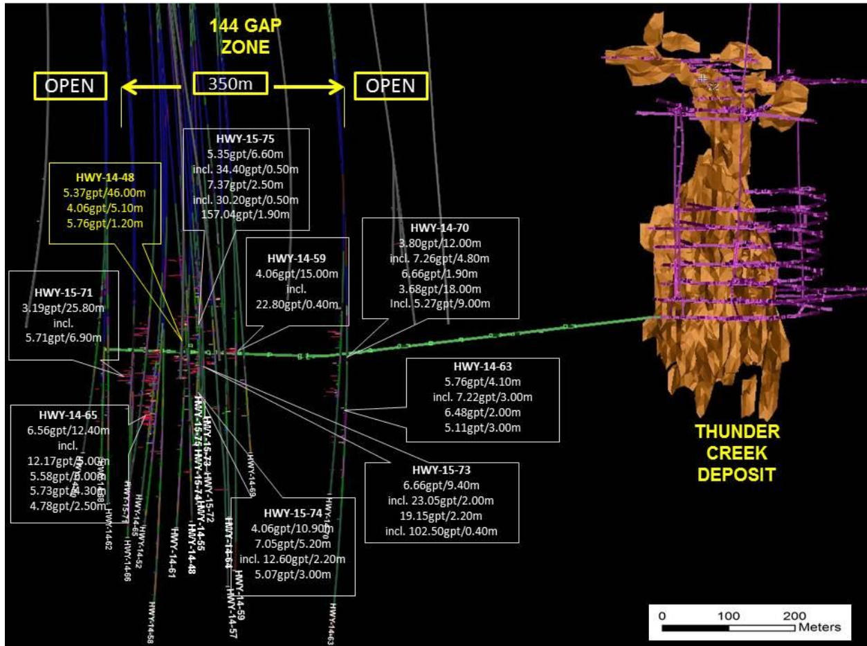
Figure 3. 3D Visual 144 Gap Zone (Looking Northwest)
