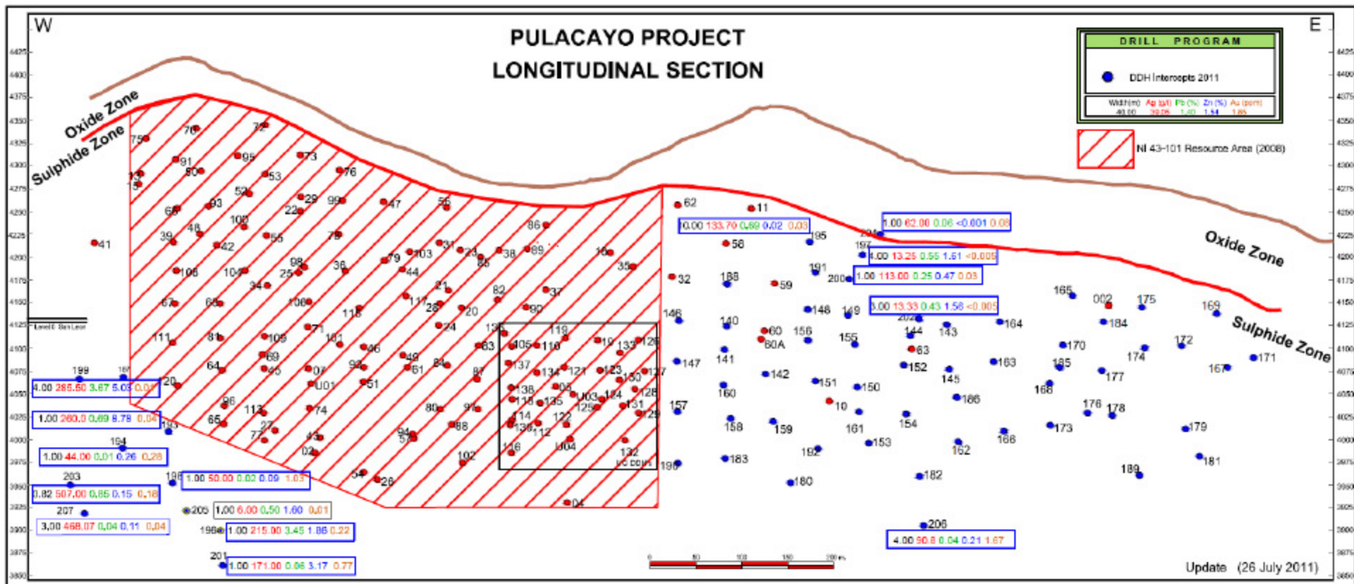
Figure 3 Pulacayo Vertical Longitudinal Section
