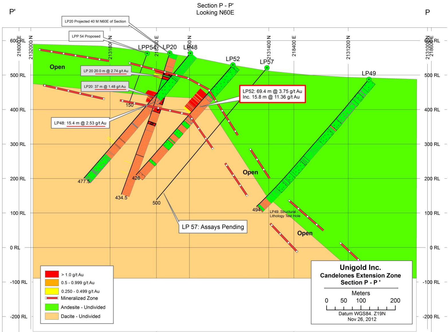
Figure 3: Section P-P'
