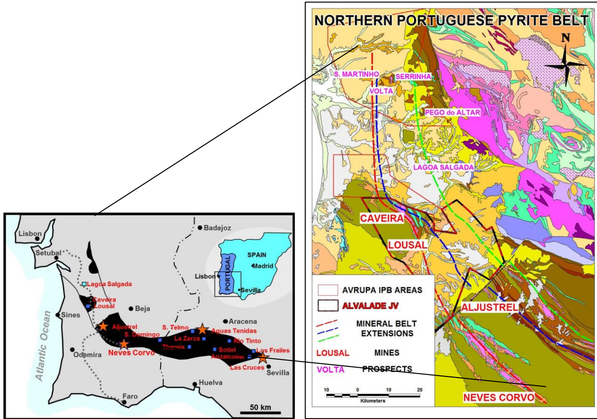
Figure 4. Avrupa IPB licenses in the Northern Portuguese Pyrite Belt. Note presence of the three main mineral trends: Neves Corvo (red), Aljustrel (blue), and São Domingos (green).
