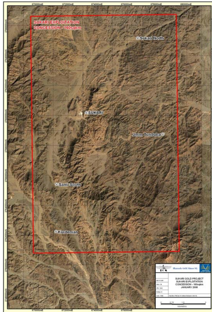
Figure 4 – Regional map of prospects and the current 160km 2 licence area.
