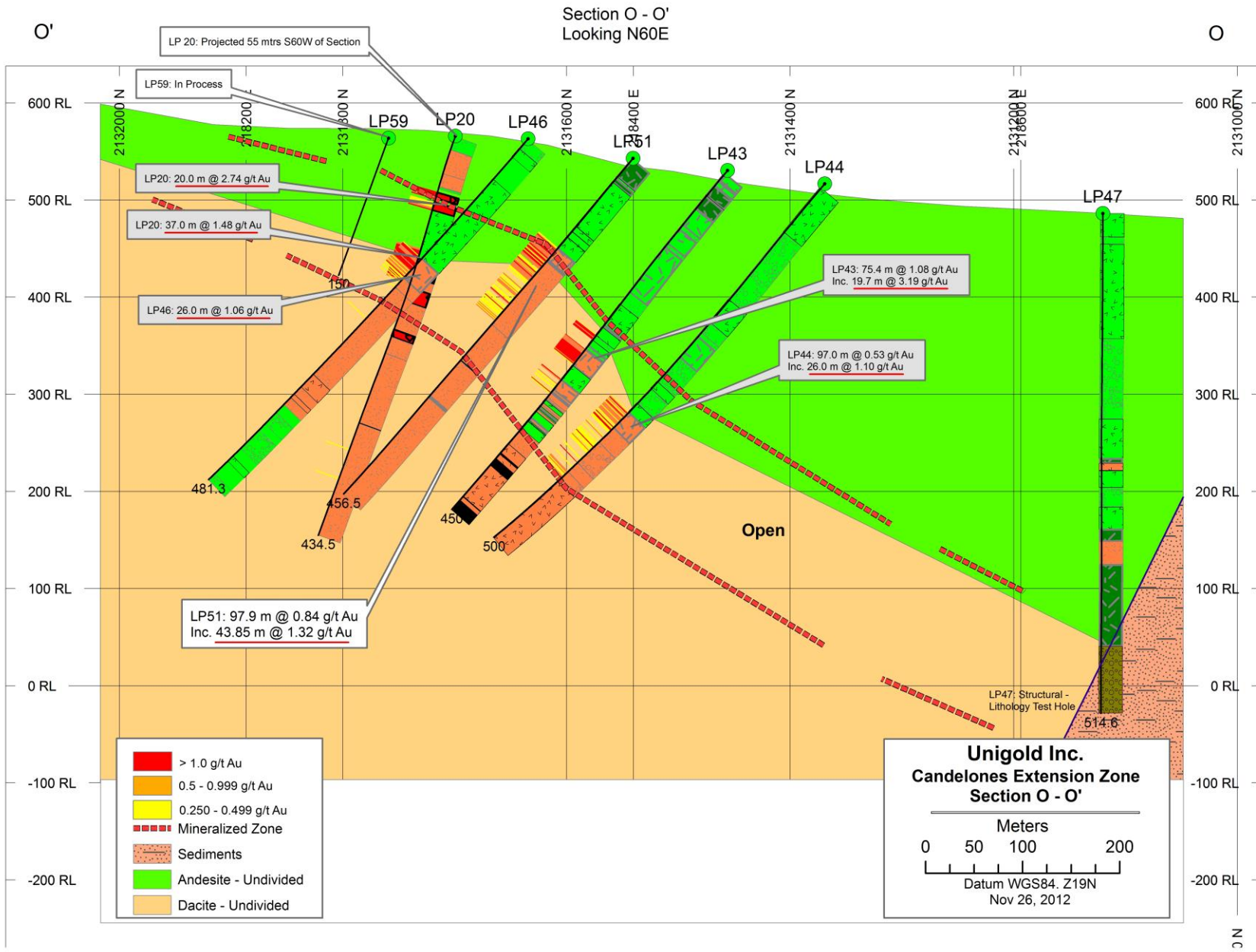
Figure 4: Section O-O'
