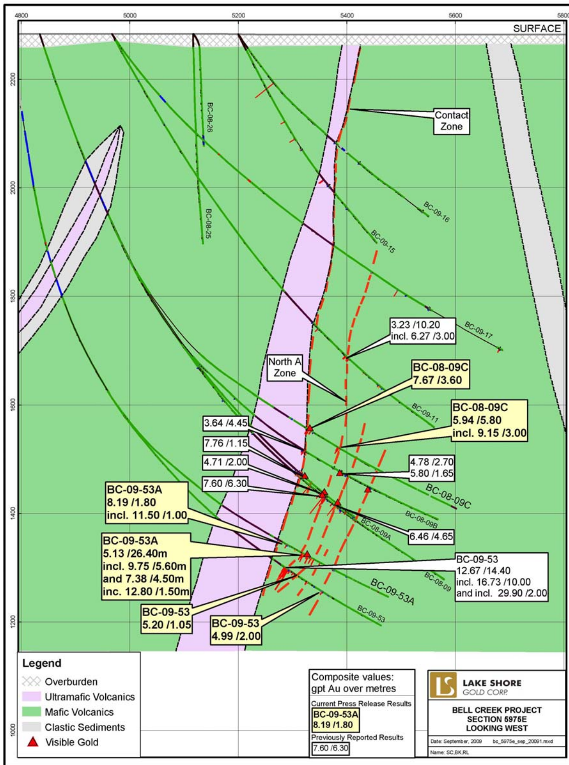
Figure 4. Cross Section (2)
