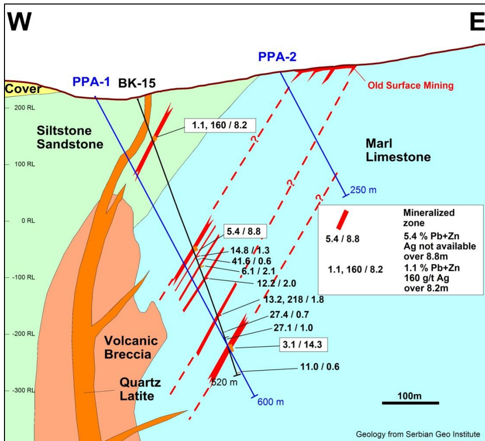
Figure 5: Parlozi section.
