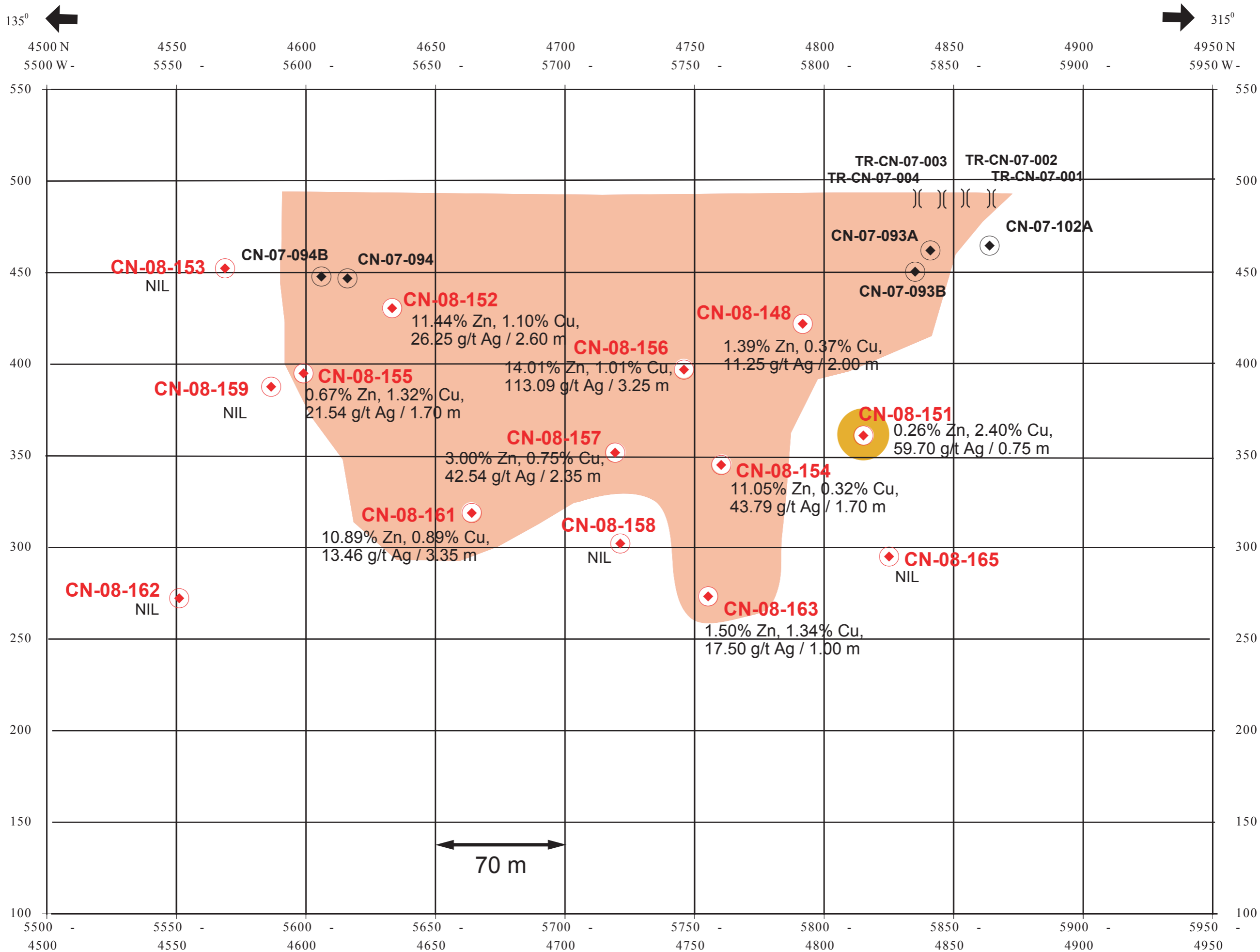
Projection longitudinale verticale de la lentille Spirit Vertical longitudinal projection of the Spirit Lens
