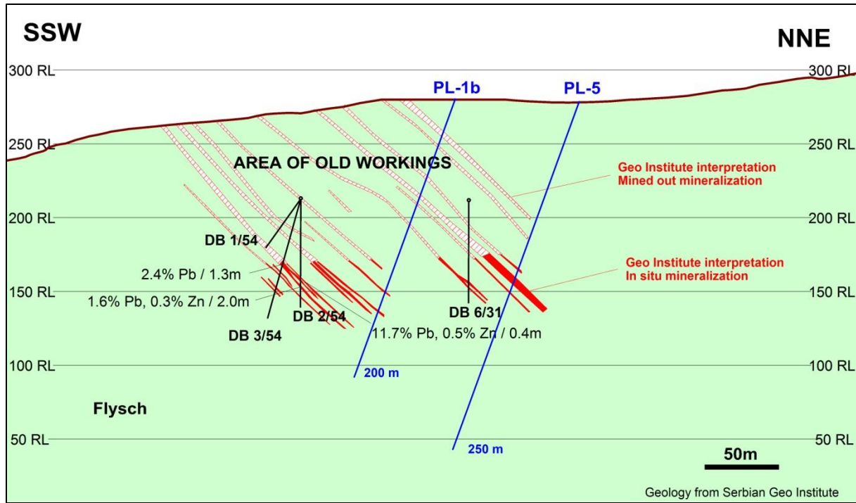
Figure 7: Plandiste section.
