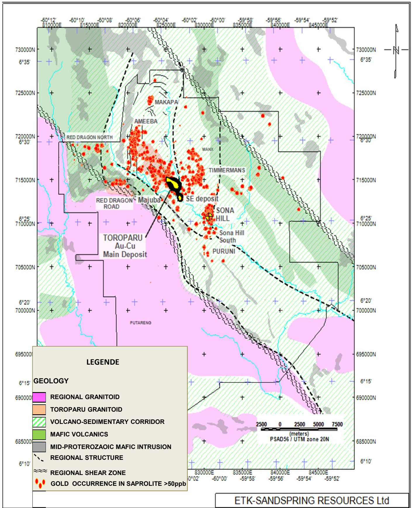
Figure 2 : Cluster of Gold anomalies around the Toroparu gold-copper deposit
