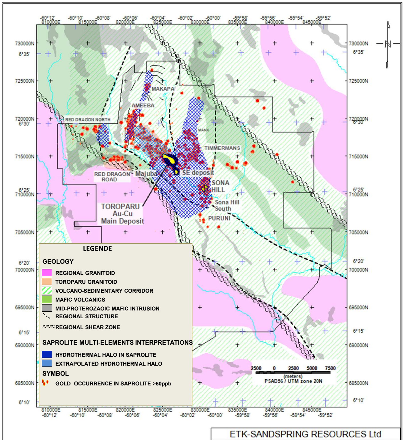
Figure 3 : Alteration Halo around the Toroparu gold-copper deposit
