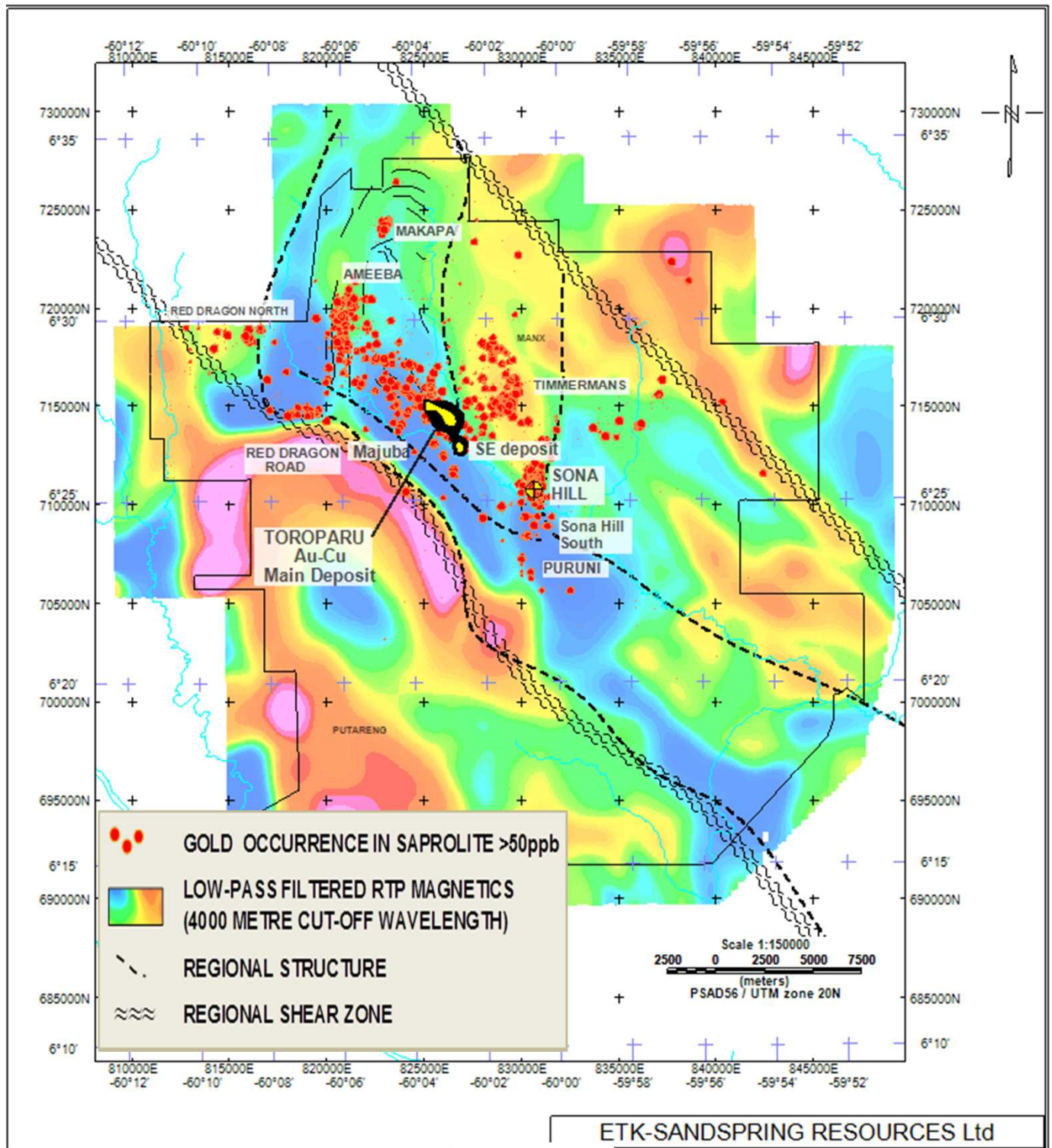
Figure 4 : Association between “Magnetic Lows” and Gold anomalous features
