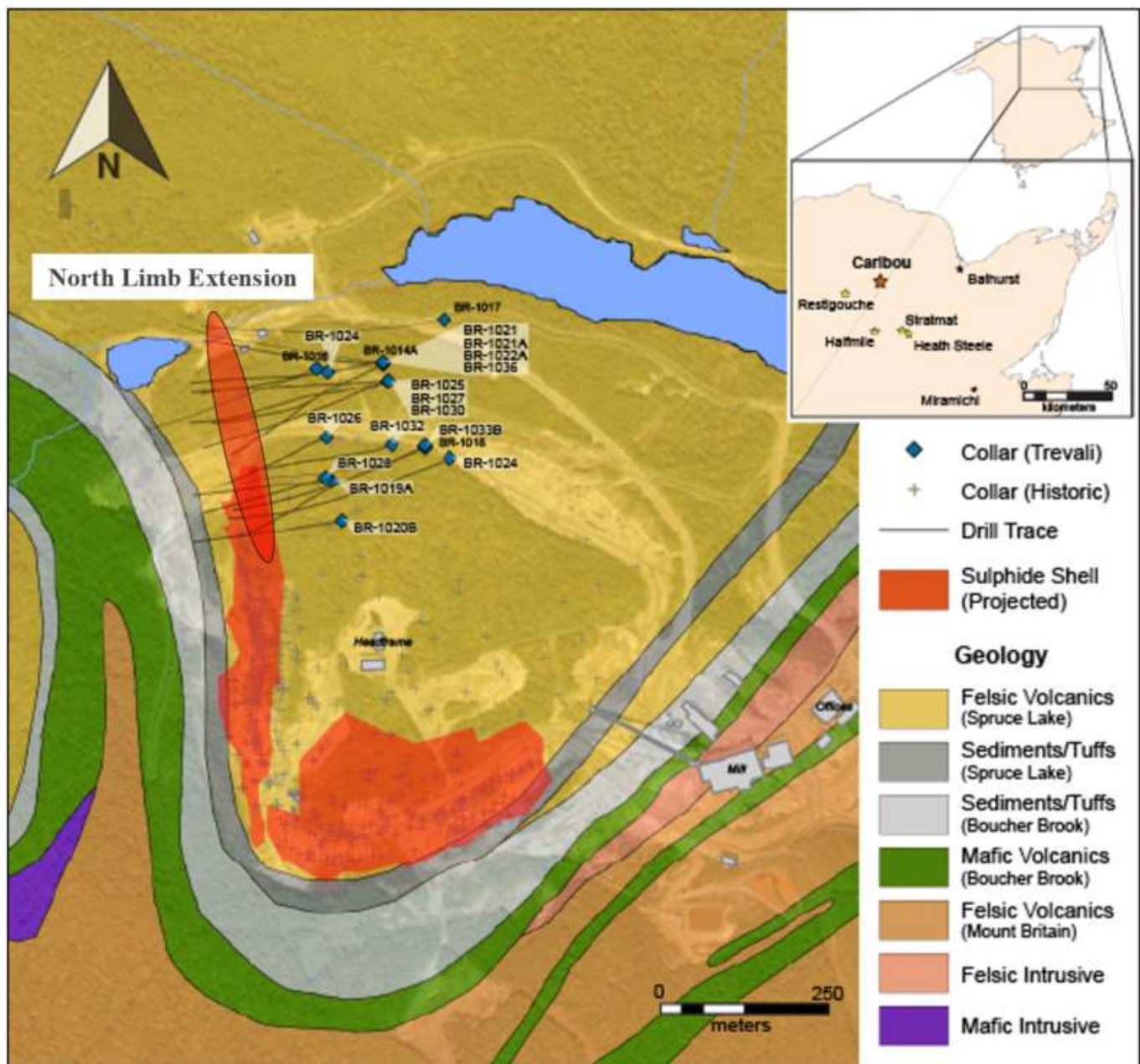
Figure 1: Geologic map of Caribou Mine area with projected North Limb extension of massive sulphide mineralization.
