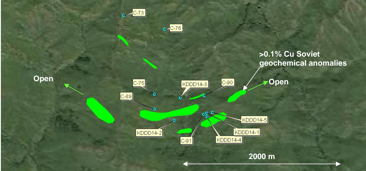
Figure 2. Location of the 2014 scout and Soviet drillholes at the Kogodai Prospect (Table 1).
