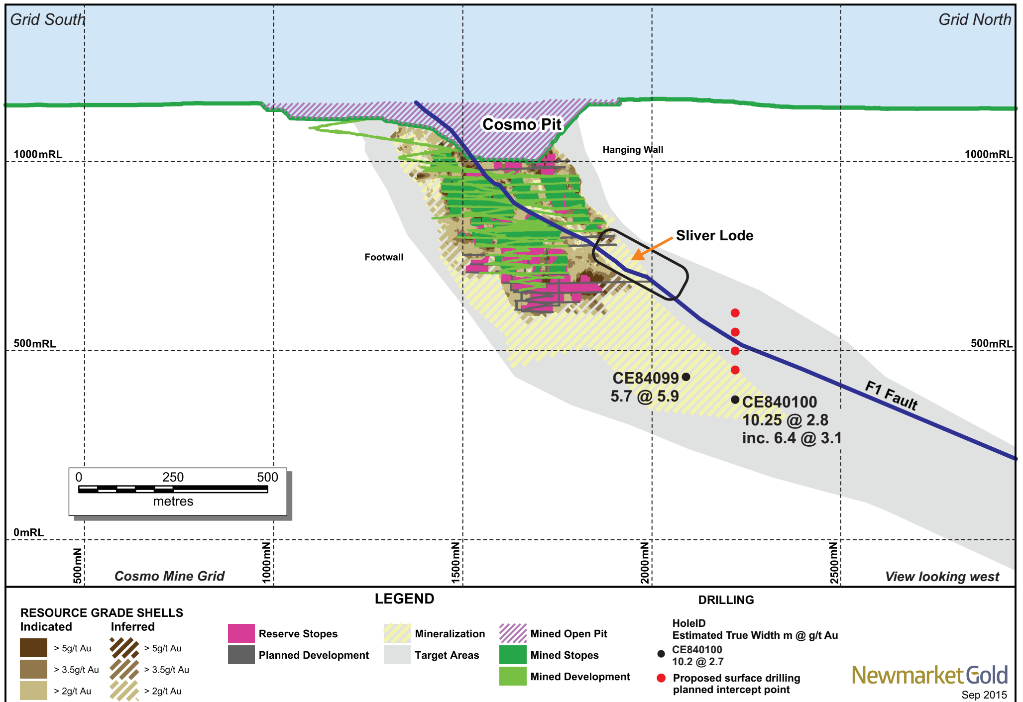
Figure 2 Longitudinal Projection of Cosmo Mine showing Drilling Areas
