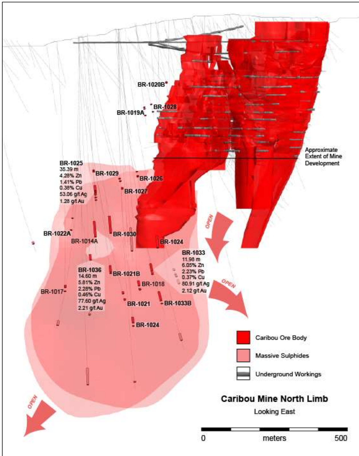
Figure 2: 3D view of the Caribou mine, looking East and illustrating geometry of the mineralization and location of recent drill hole intercepts.
