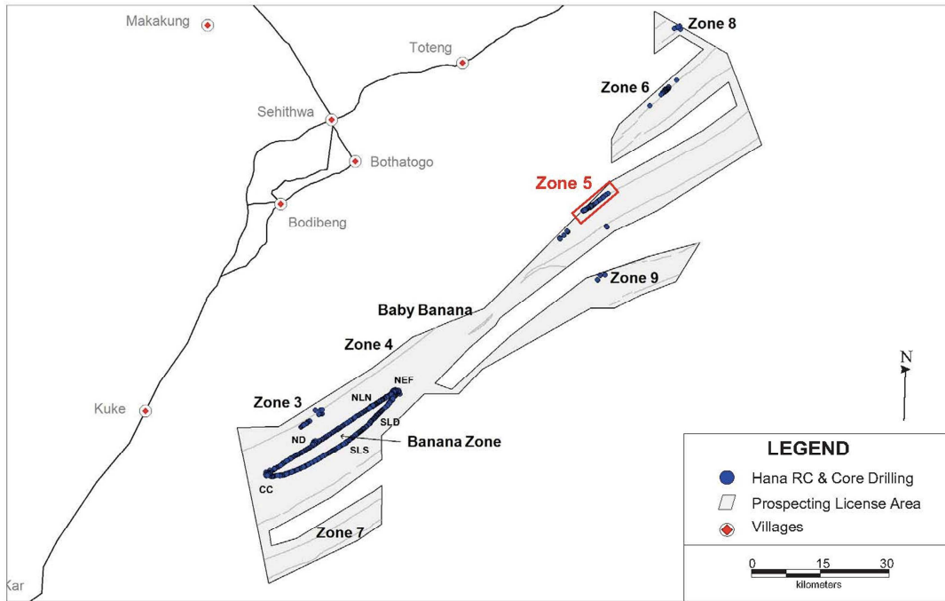
Figure 1: Location of Zone 5 Drilling Results at the Ghanzi Project
