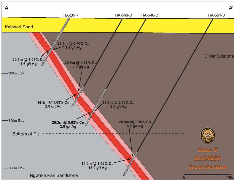
Figure 3: Cross-section through section N125850 (Zone 5)
