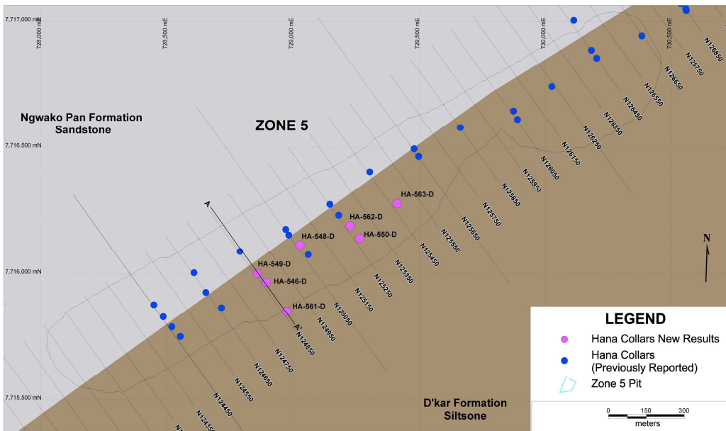
Figure 2: Drill Hole Location of Zone 5, Including Sections N124850 to N125450
