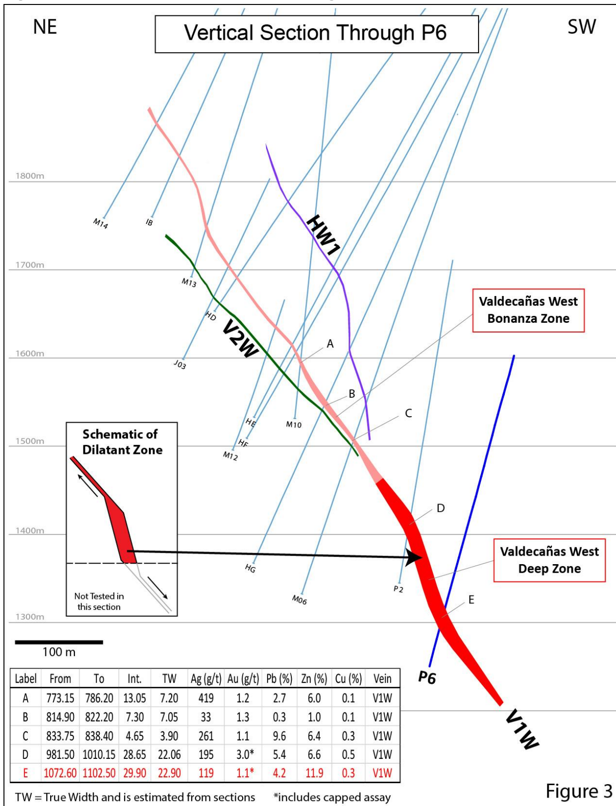
Figure 3: Valdecañas Vein Cross Section through P6
