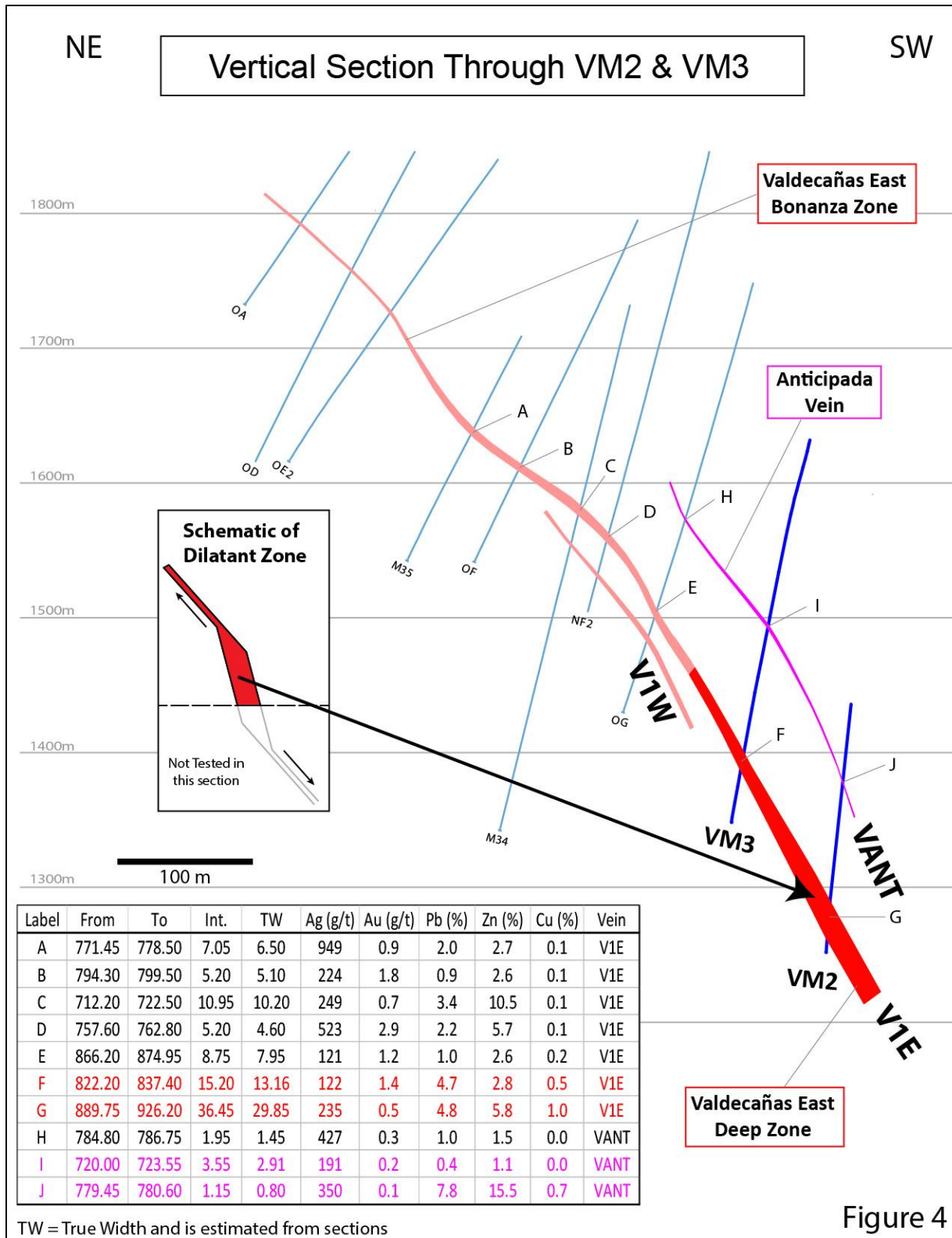
Figure 4: Valdecañas Vein Cross Section through VM2 & M3
