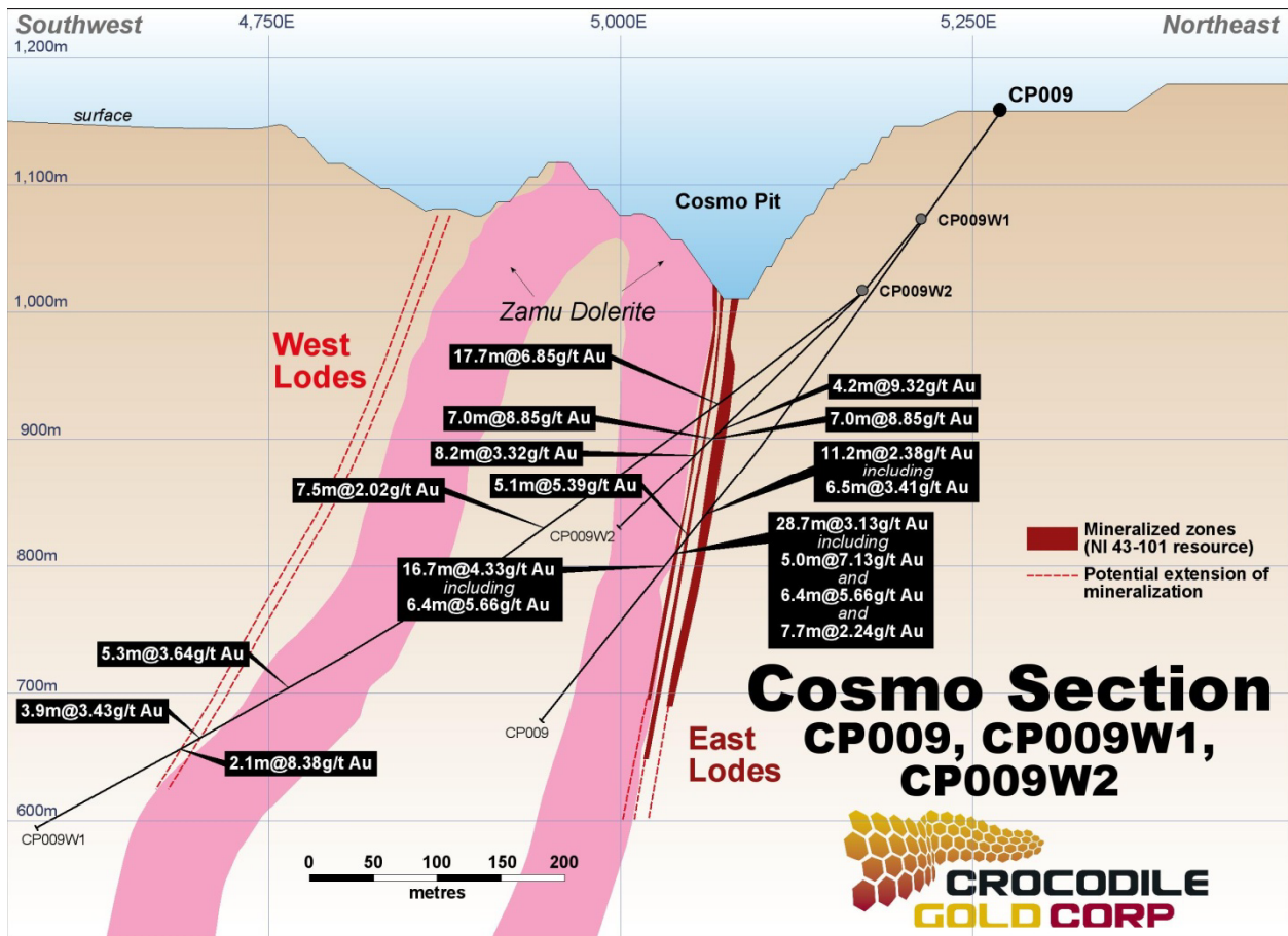
Figure 5: Cosmo Section – Holes CP009, CP009W1 and CP009W2
