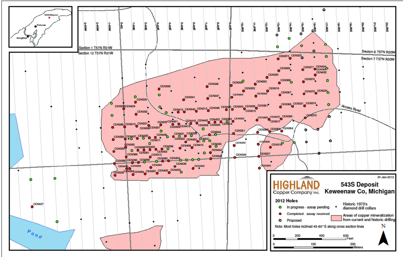
FIGURE 1. Drill hole locations at the 543S deposit. All holes are inclined at 45-80 degrees to the south along the section lines except holes CEN306 and CEN307 that are inclined to the west.
