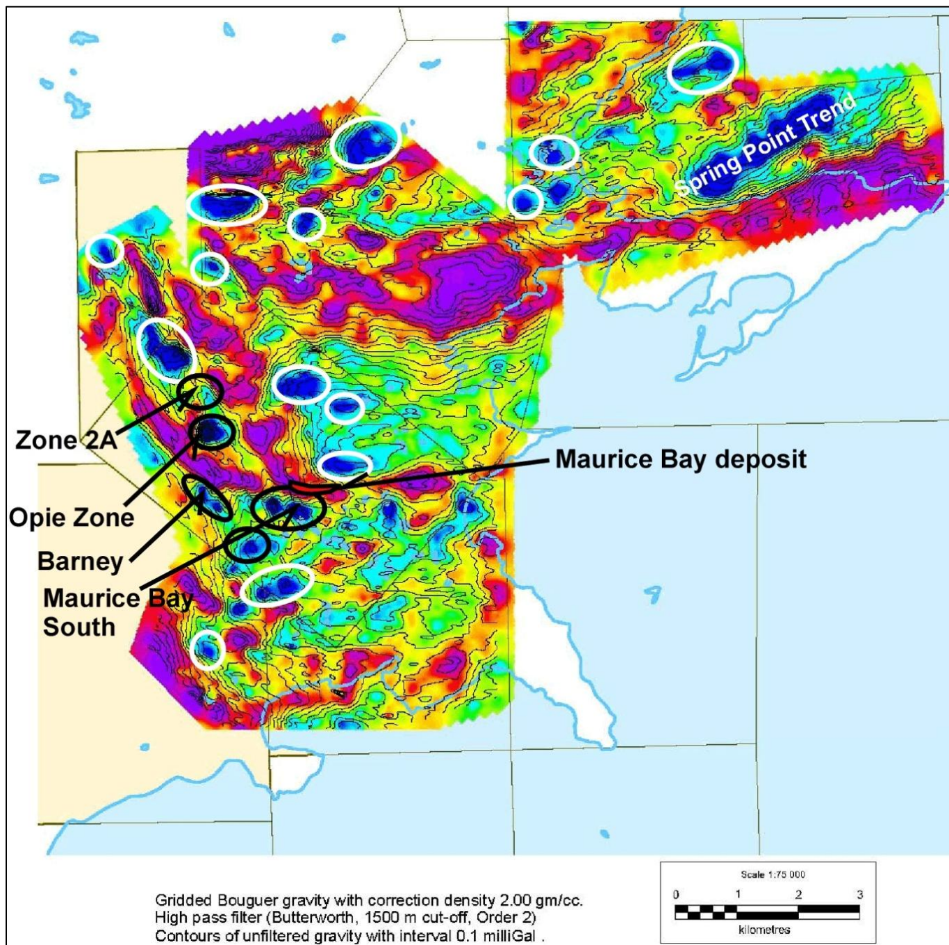
Figure 2: NW Athabasca Project Gravity Survey. Numerous gravity lows have been identified on the project, with 15 of them untested by previous drilling (white outlines). 2012 work areas are outlined in black.
