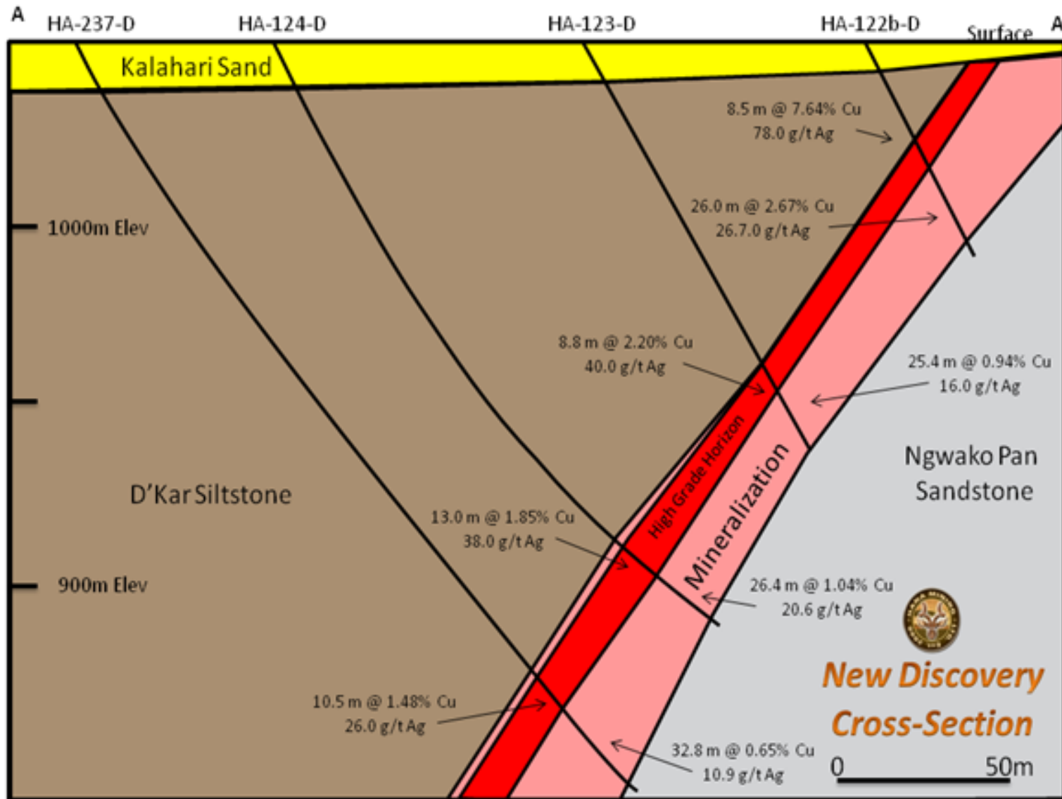
Figure 3: Cross-section through section 50250 (North Limb)
