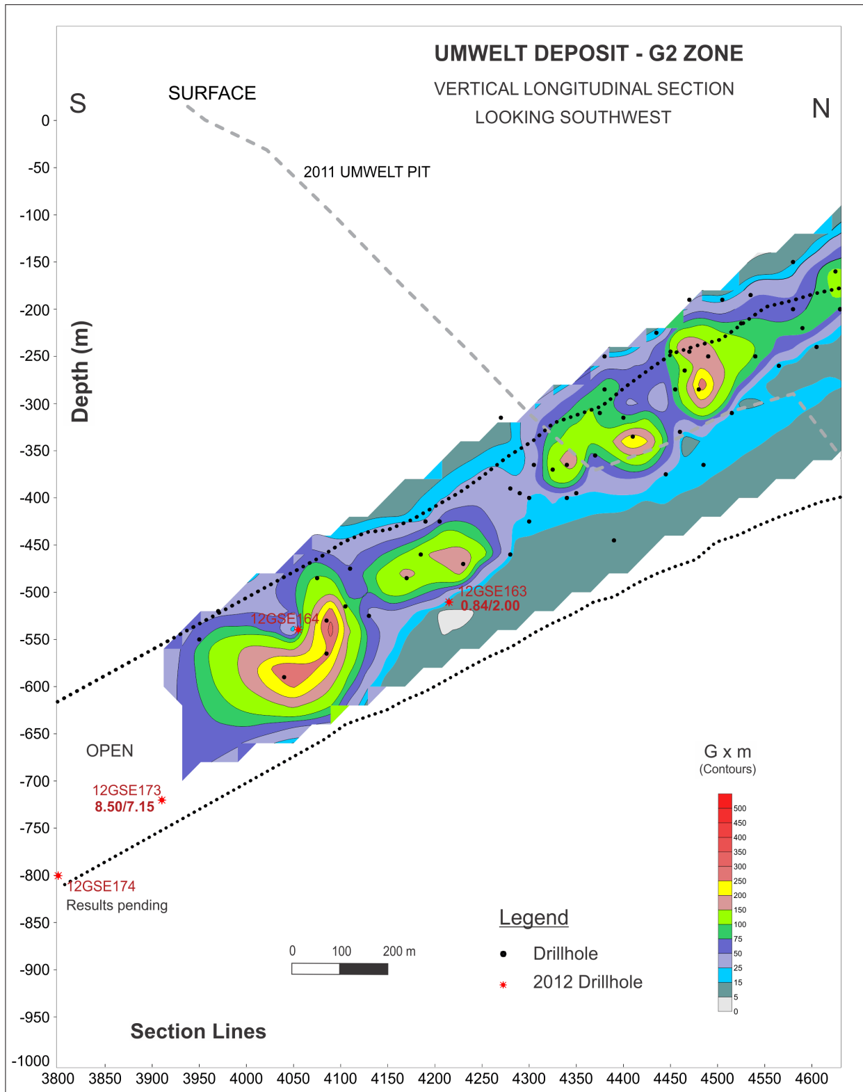
Figure 3: Umwelt Longitudinal Section
