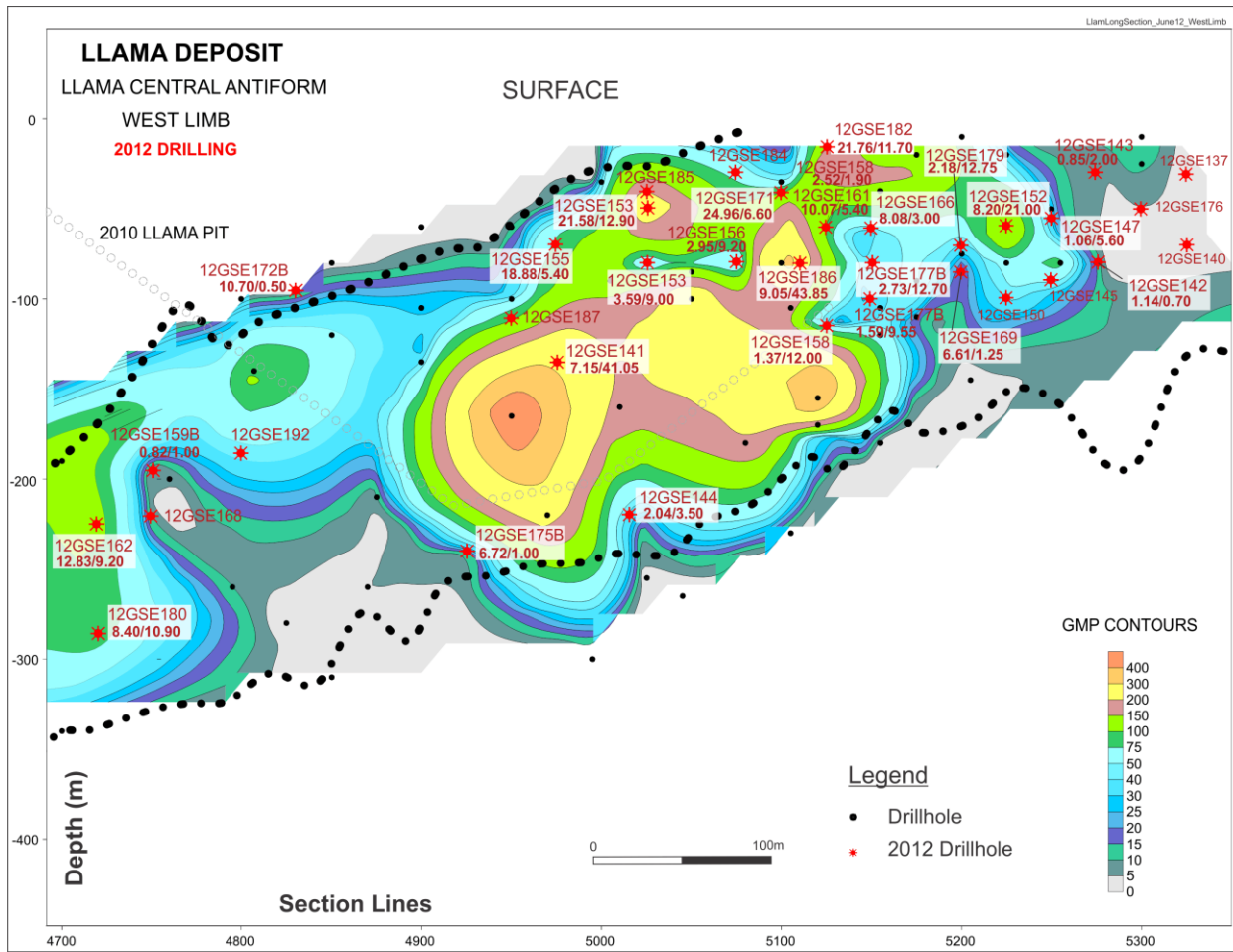
Figure 2: Llama West Limb Longitudinal Section
