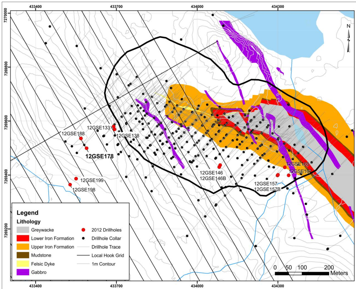
Figure 4: Goose Hook Area Plan Map
