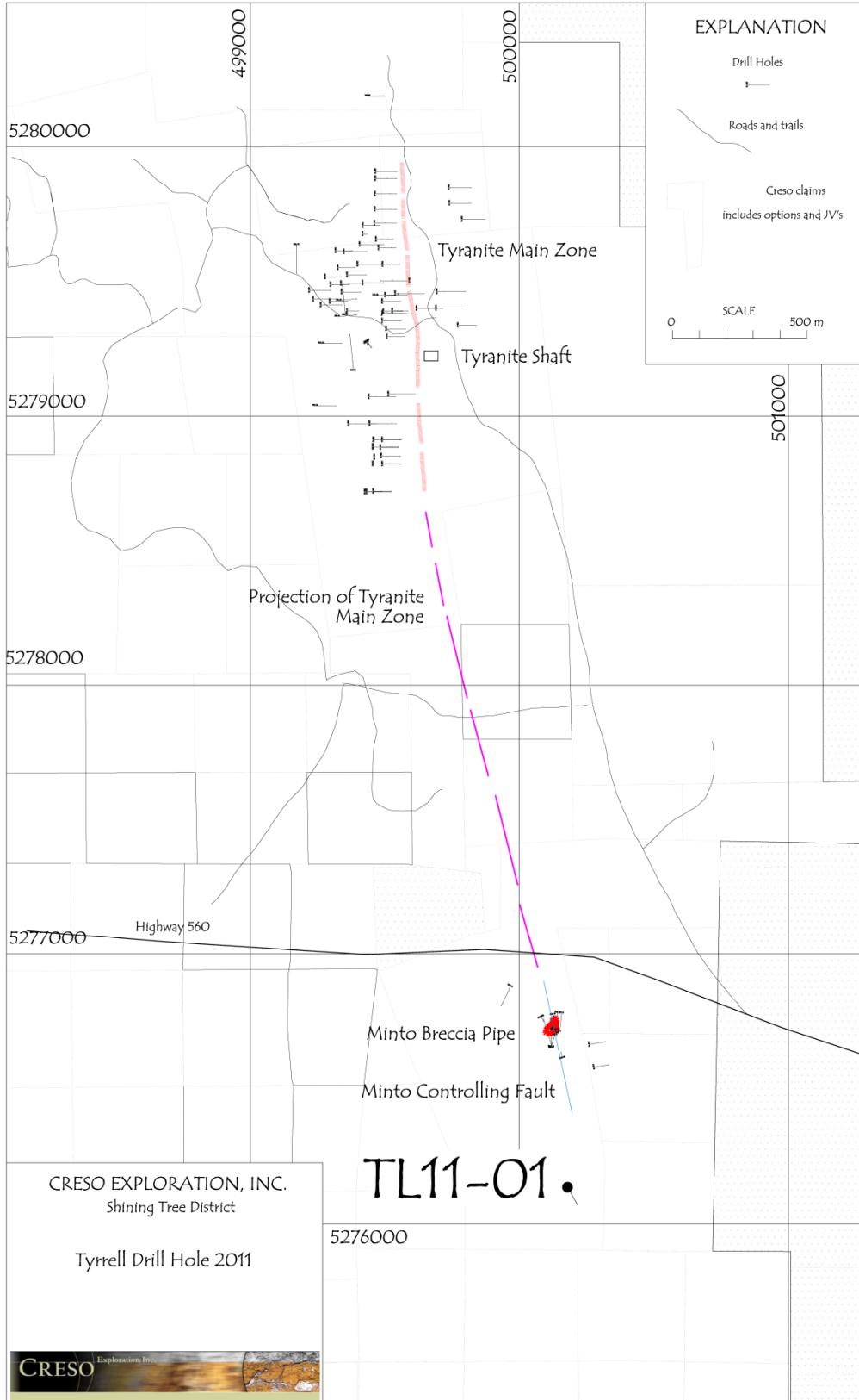
Figure 1. Location of TL11-01 drill hole at Tyrrell, Shining Tree District, Ontario
