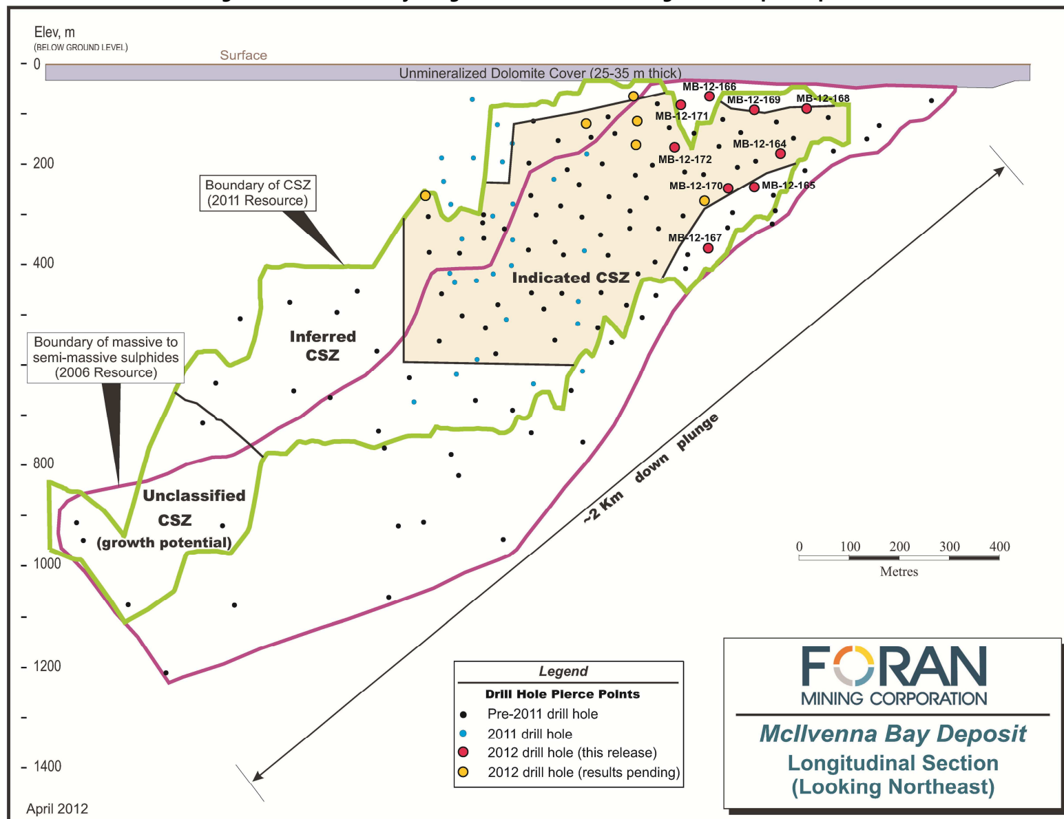
Figure 1: McIlvenna Bay Longitudinal Section showing drill hole pierce points.
