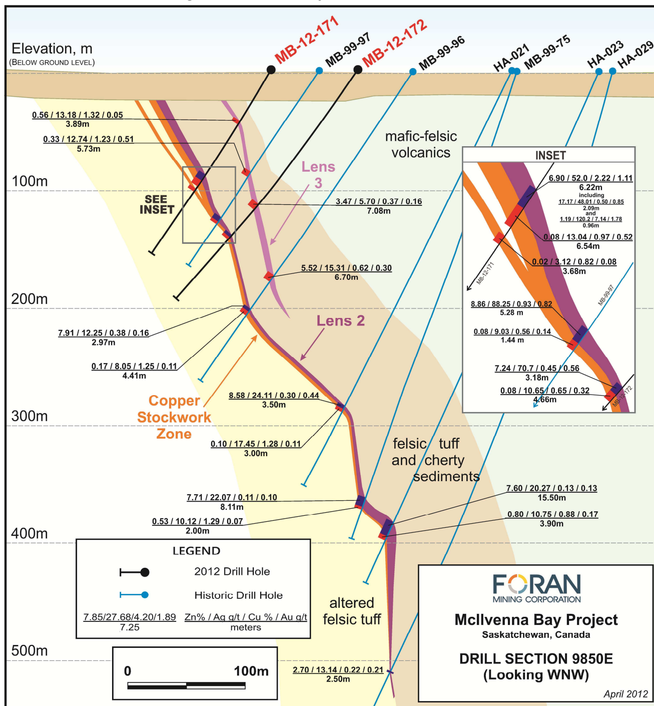
Figure 2: McIlvenna Bay Cross Section 9850E.
