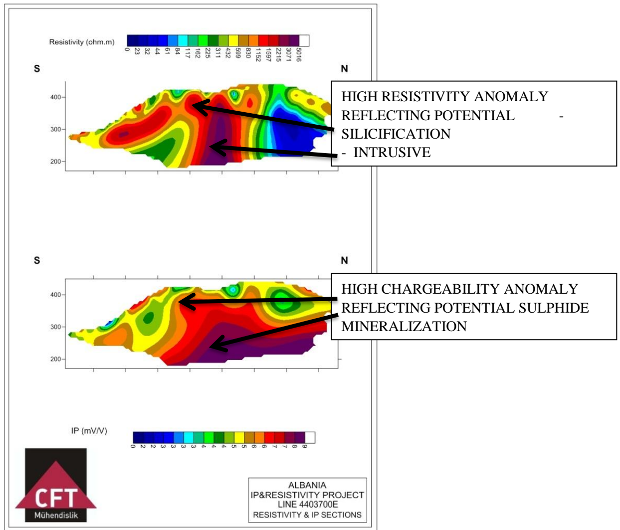
TYPICAL RESISTIVITY AND CHARGEABILITY PROFILES
