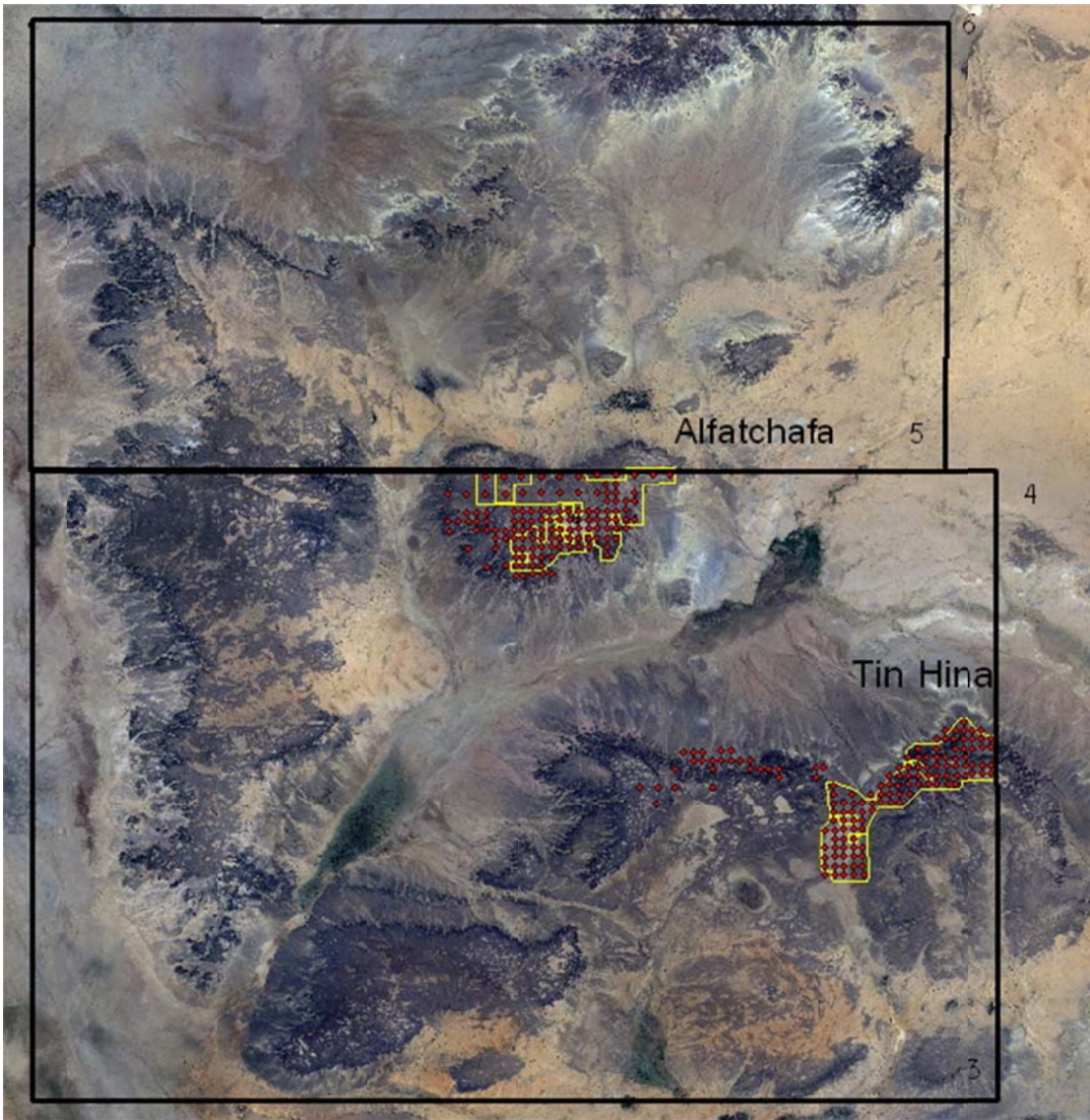
Figure 4: Overview of the Tilemsi project, with drill holes in red, ore polygons in yellow and the outline of license areas (black lines). See website for Report.
