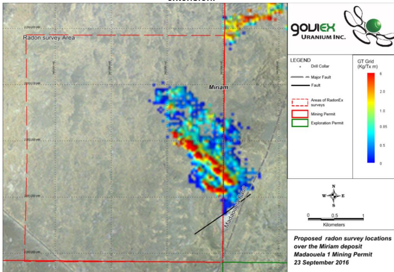
Figure 2. Area map showing proposed radon survey locations over Miriam extension.
