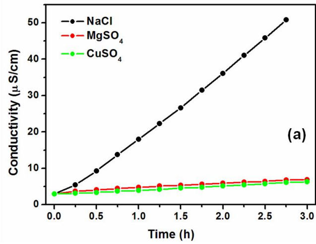
Figure 1 (a) shows the penetration processes of different ionic compounds through the GPURE GPM membrane, and (b) shows the GPURE GPM 6cm x 6cm membrane.
