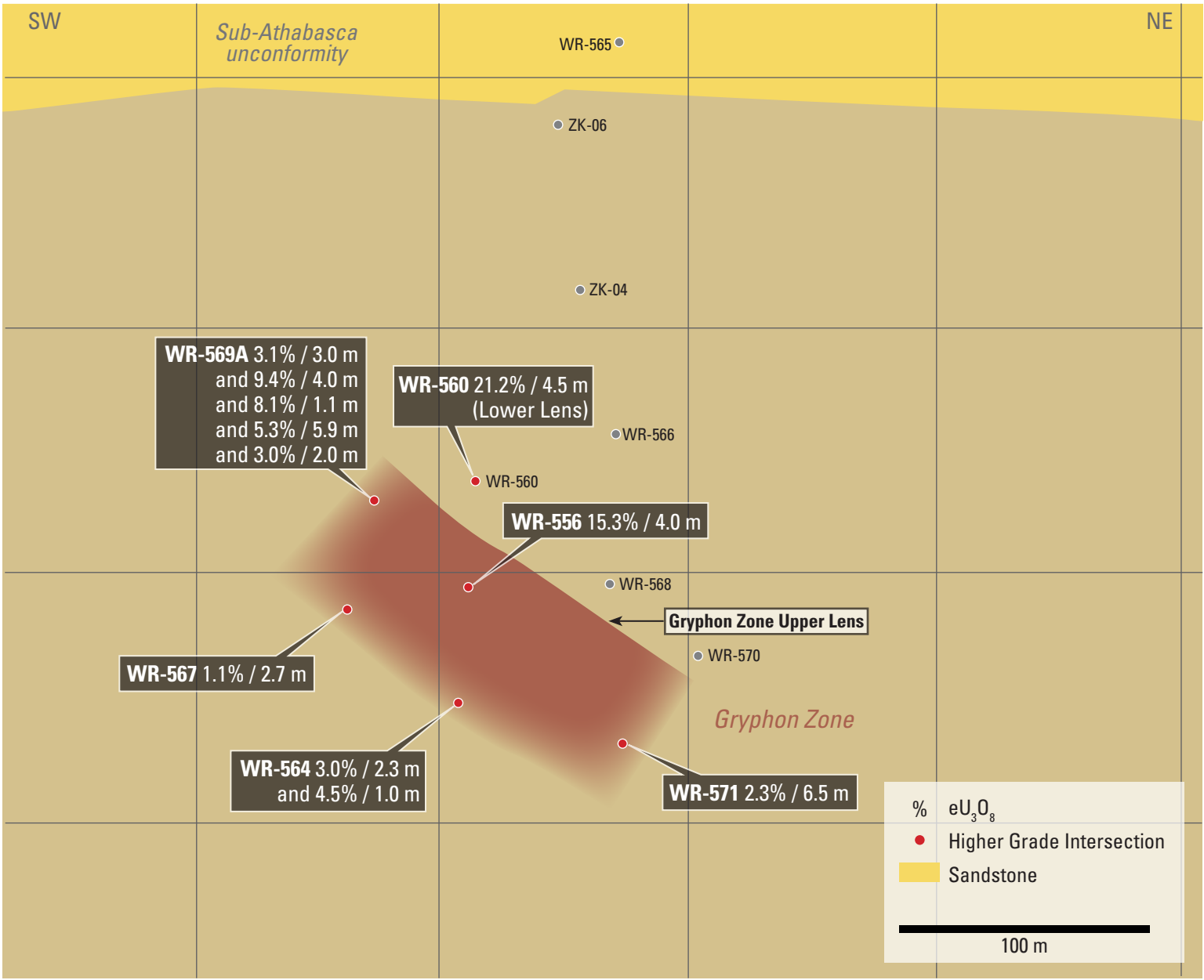
Gryphon Zone Upper Lens Longitudinal Section July 29, 2014
