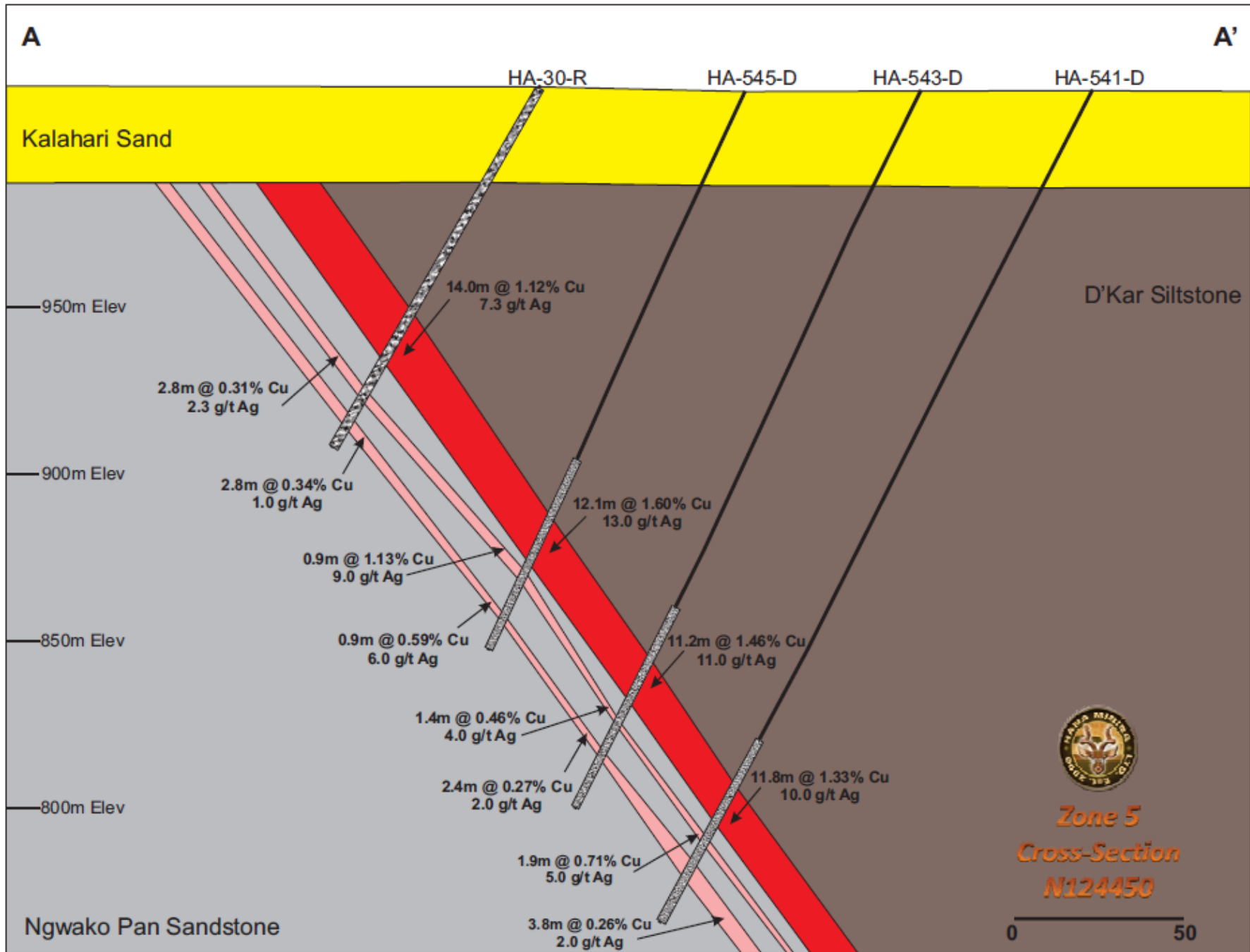
Figure 3: Cross-section through section 124450 (Zone 5)
