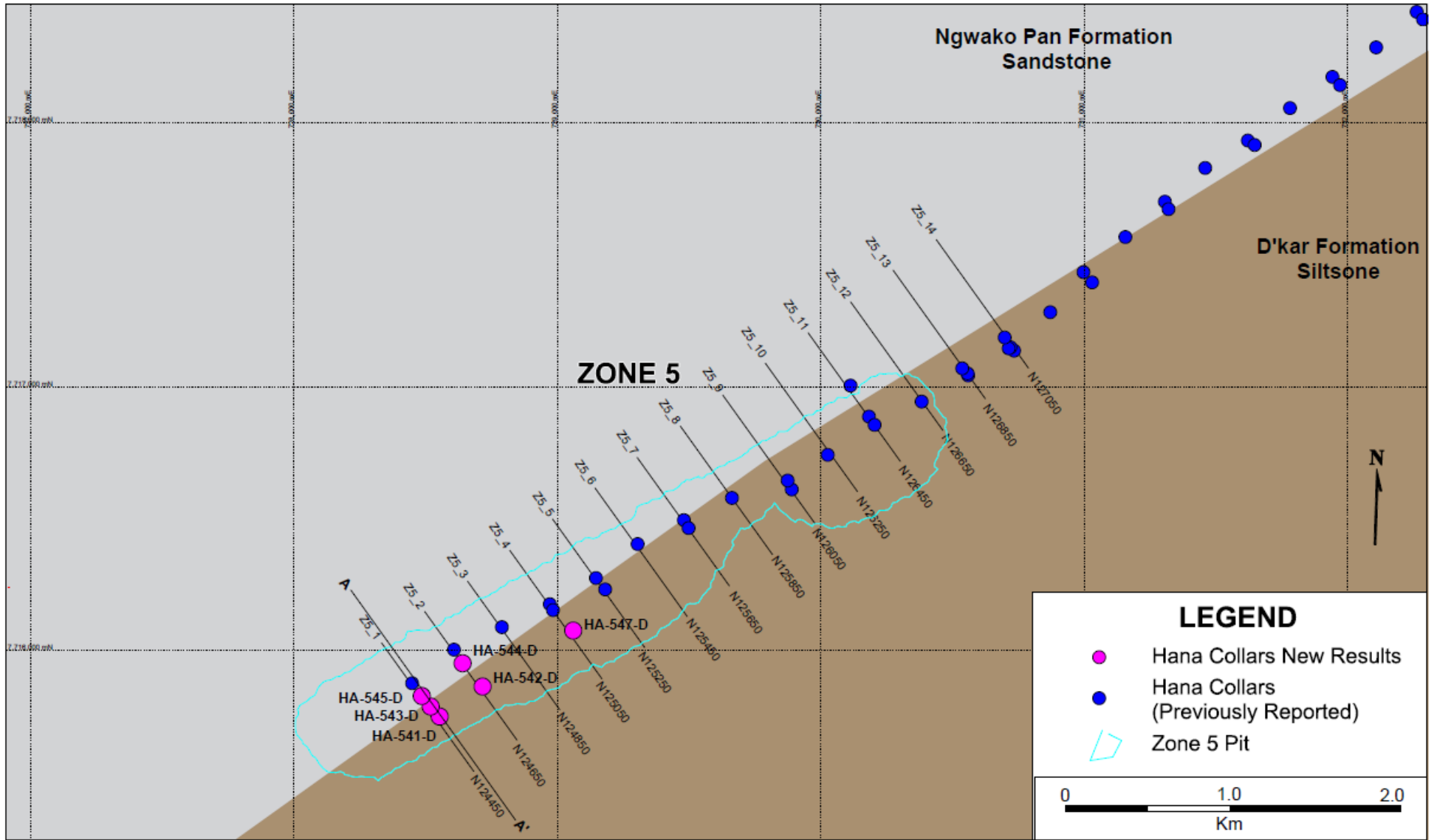
Figure 2: Drill Hole Locations at Zone 5, Sections 124450 - 125050
