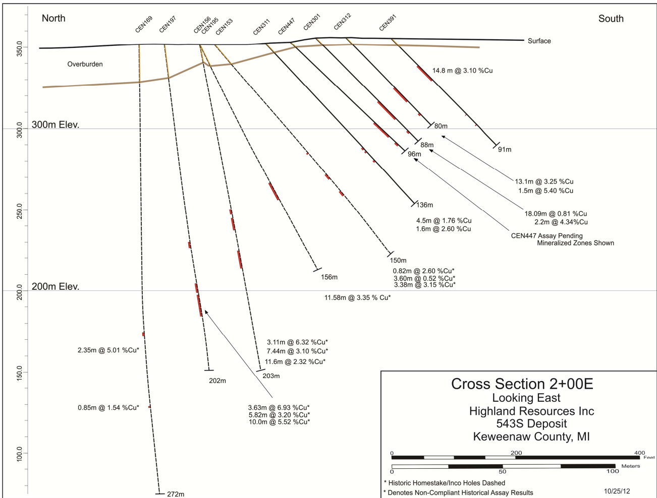
FIGURE 2. Cross section 200E, looking east, 543S deposit. Holes CEN 306 and CEN 307 are inclined to the west and are not shown.
