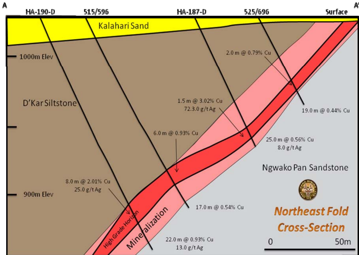
Figure 3: Cross-section through section 69600 (Northeast Fold)
