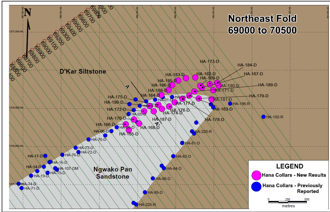
Figure 2: Drill Hole Location of North Limb, Sections 69000 to 70500
