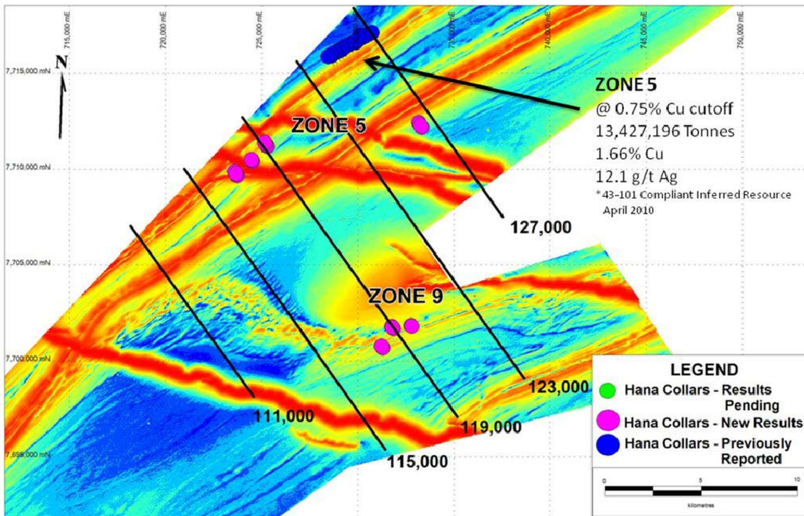
Figure 3. Location of drilling at Zones 5 and 9 with airborne magnetics (red areas are magnetic highs)
