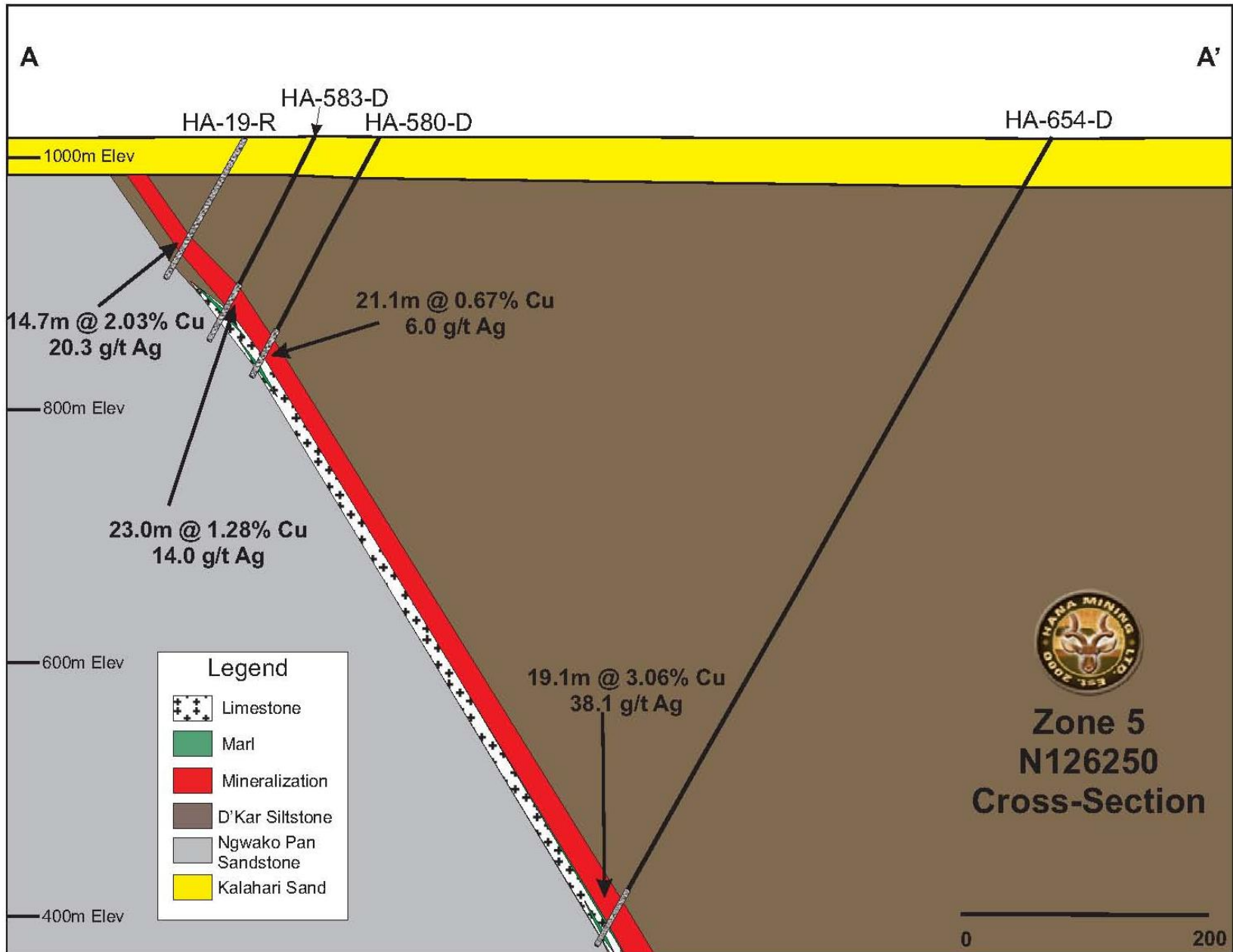
Figure 3: Cross-section through N126250 at Zone 5 showing exploration deep drilling
