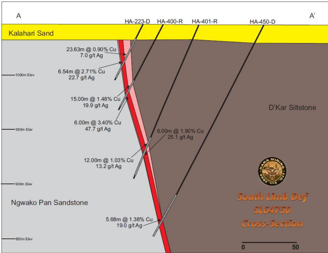
Figure 3: Cross-section through section 64750 (South Limb Definition)
