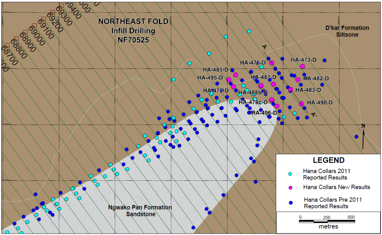
Figure 2: Drill Hole Location of Northeast Fold, Sections 70125-70725
