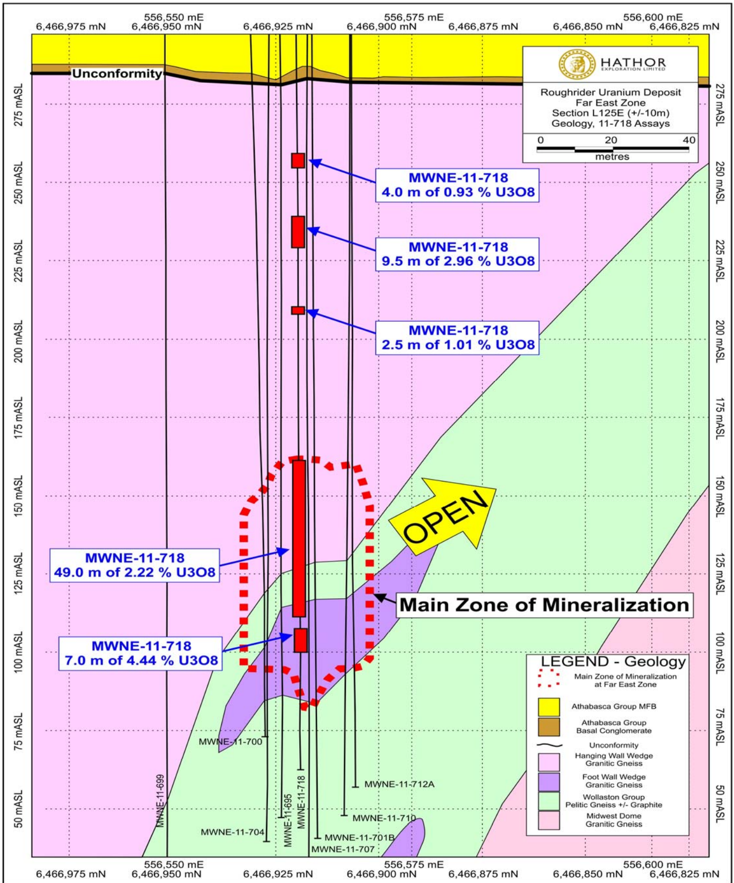
Figure 2: Cross section showing composited assays for drill hole MWNE-718, and the spatial relationship between the main zone of mineralization at Far East, and the new, shallower zone of mineralization near the unconformity. Grid Line 125 East ( \pm 10 m), view northeast. Modified and updated from Figure 3 in the Company's news release dated September 20, 2011.
