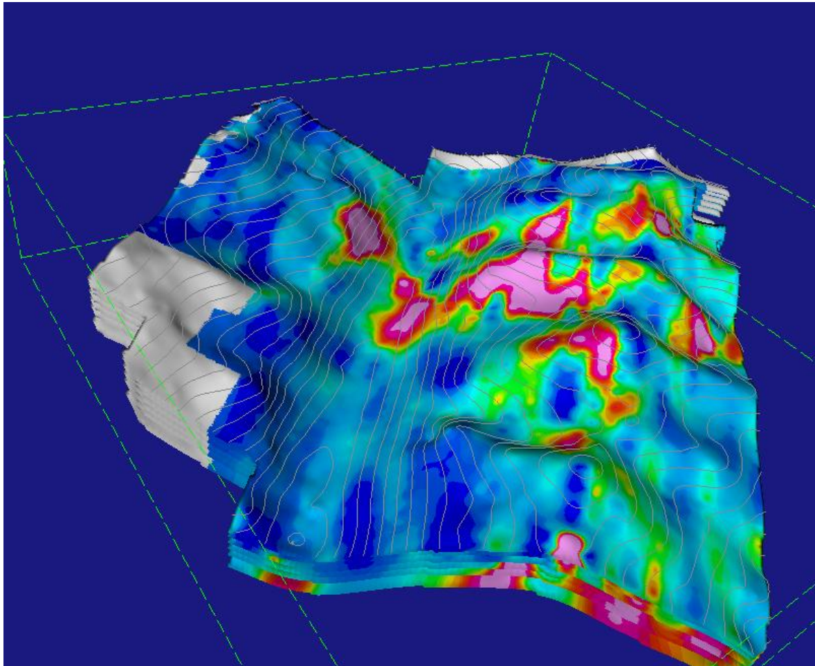
Figure 1. The 3D chargeability model for the Chanape grid at 20-50-100-150-200-300 meters depth; looking NE. The strongest responses are identified by red and pink colours.
