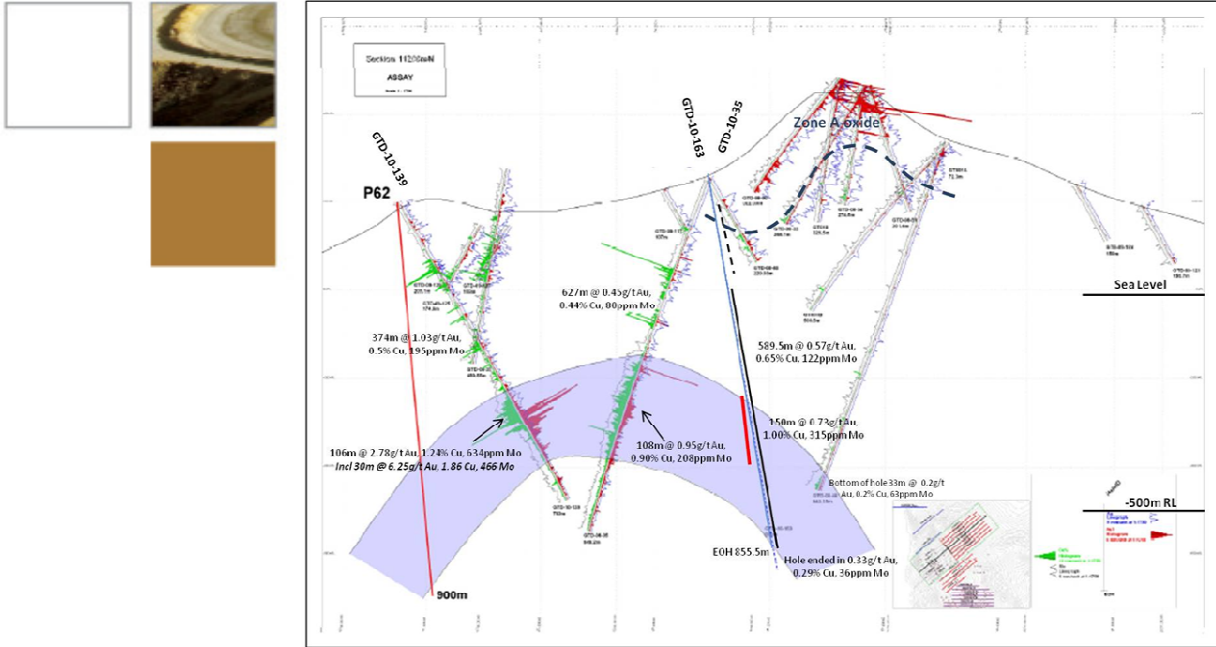
Cross section through the central part of the porphyry copper-gold mineralised system showing intercepts in holes GTD 139, 35 and 163.
