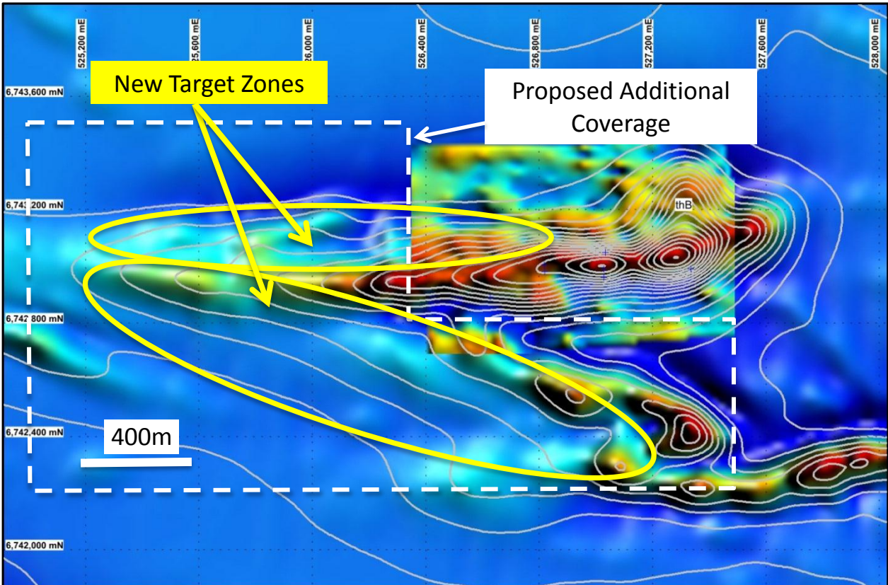
Figure 3 – Proposed additional coverage by ground gravity at Axehead to explore new target zones.
