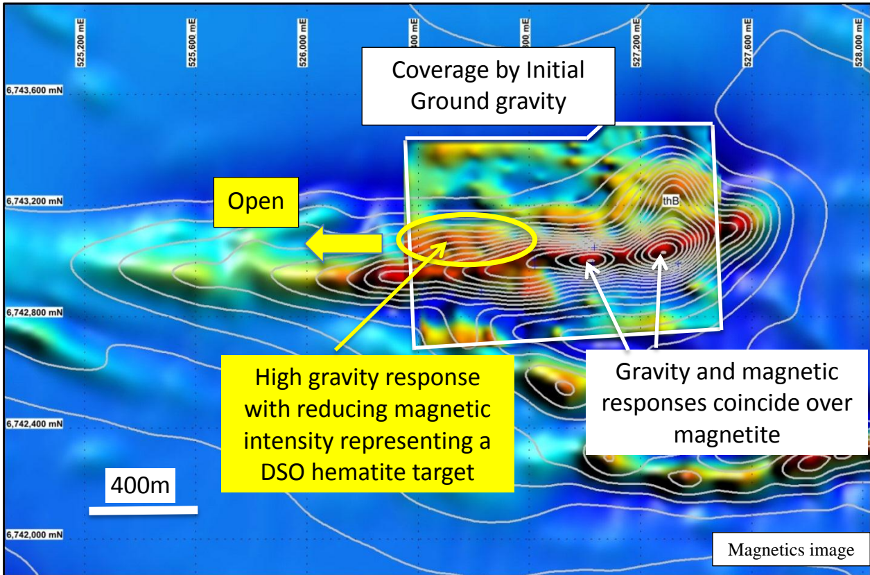
Figure 2 – Axehead prospect: Contours show magnetic intensity; Gravity response indicated by colour – red is high
