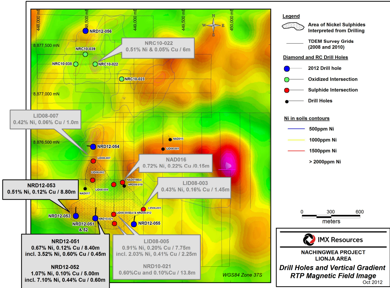
Figure 2. Lionja drilling location with significant intersections
